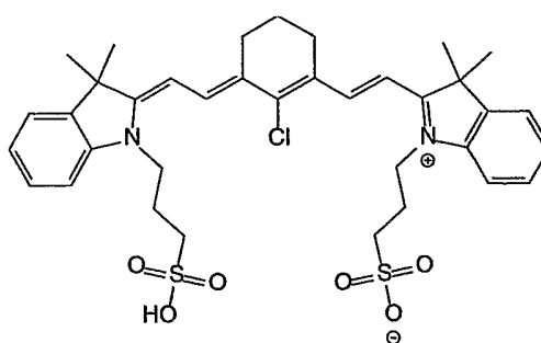
IR Dye structure:
