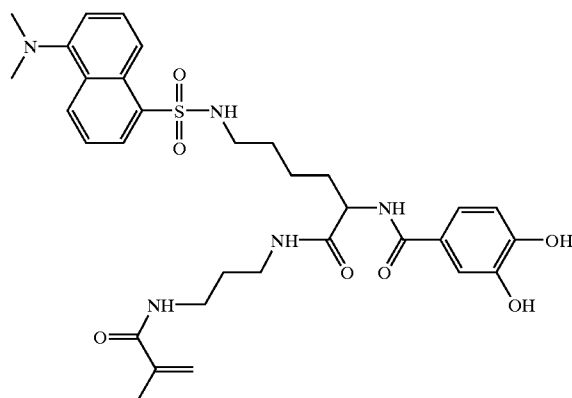
DANSYL-catechol monomer
