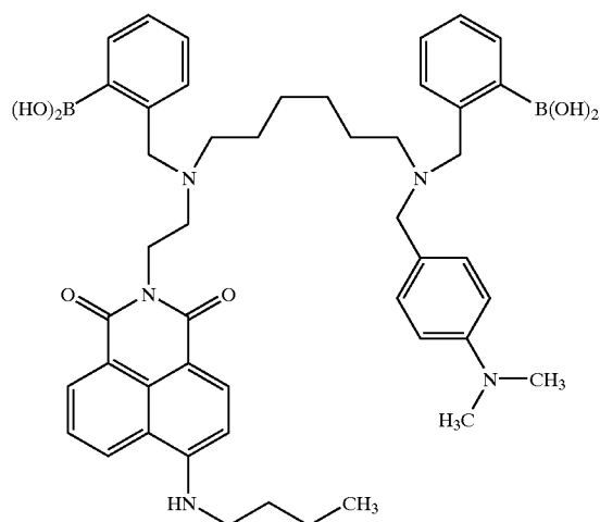
nBuF-hexa-Q bis-boronate
