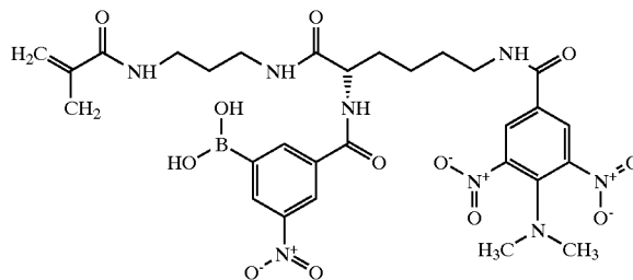
DANSYL-catechol monomer
