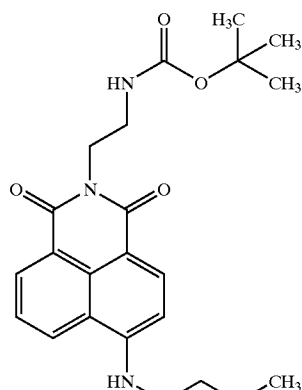
N-2-(tert-butoxycarbonyl)aminoethyl-4-butylamino-1,8-naphthalimide
