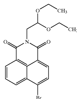
N-(2,2-diethoxyethyl)-4-bromo-1,8-naphthalimide
