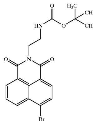
N-2-(tert-butoxycarbonyl)aminoethyl-4-bromo-1,8-naphthalimide
