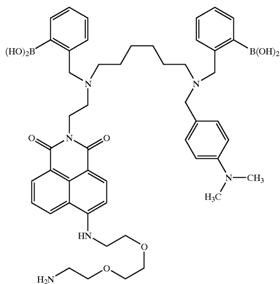
AminoethoxyF-hexa-Q bis-boronate
