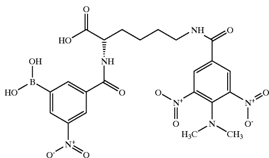
N-α-(3-boronato-5-nitro)benzoyl-N-ε-(4-dimethylamino-3,5-dinitro)benzoyllysine
