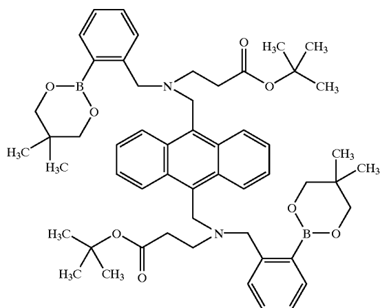
9,10-bis[N-[2-(5,5-dimethylborinan-2-yl)benzyl]-N-[2-(tert-butoxycarbonyl)ethylamino]methyl]anthracene
