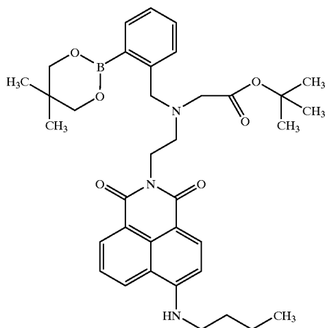
N-2-[(tert-butoxycarbonyl)methyl]-2-[2-(5,5-dimethylborinan-2-yl)benzyl]aminoethyl-4-butylamino-1,8-naphthalimide
