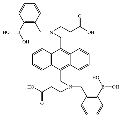
9,10-bis[N-(2-boronobenzyl)-N-[3-(propanoyl)amino]methyl]anthracene
