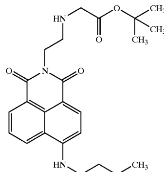
N-2-[(tert-butoxycarbonyl)methyl]aminoethyl-4- butylamino-1,8-naphthalimide
