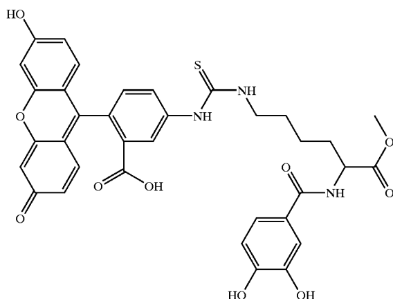
Flourescene-catechol adduct
