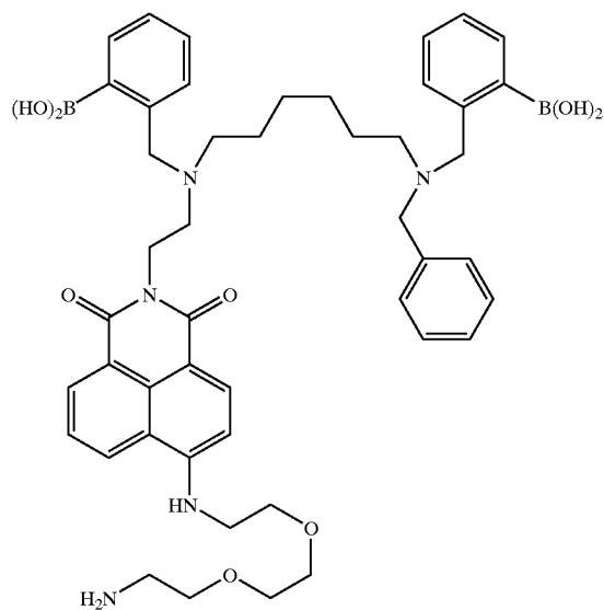
AminoethoxyF-hexa-C bis-boronate
