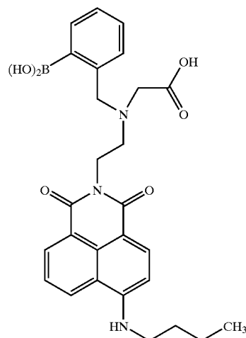
nBuF mono-boronate
