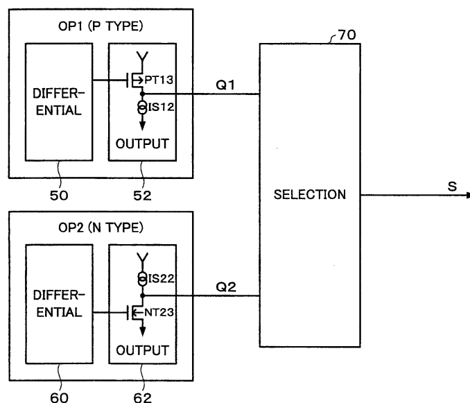
OPERATIONAL AMPLIFIER CIRCUIT
