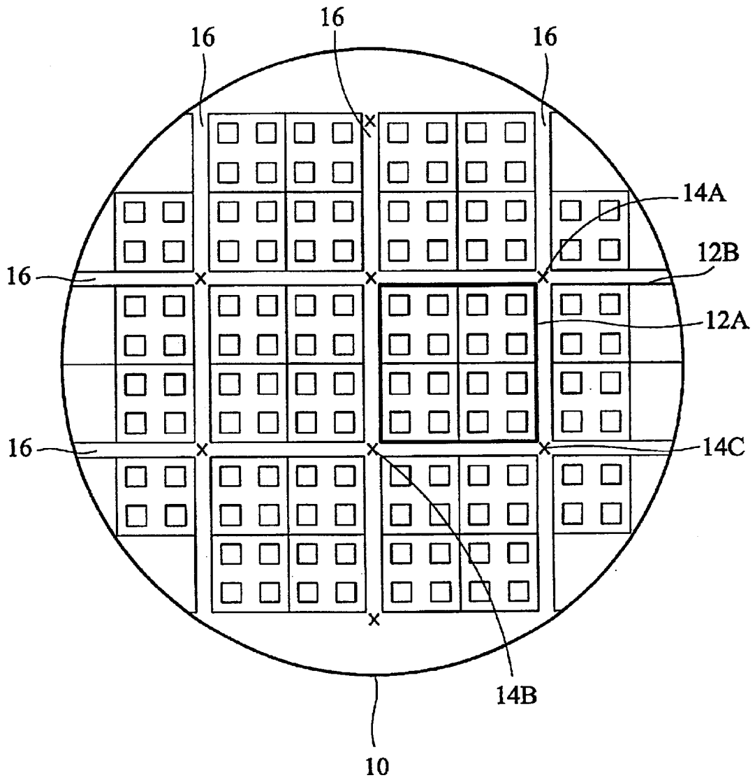
FIG. 1 (PRIOR ART)
