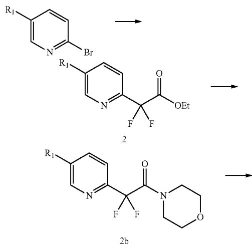
Scheme 2. Synthesis of ketone 3
