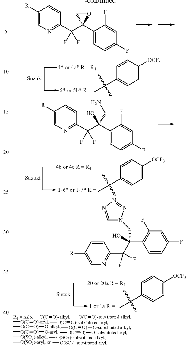
Scheme 3. Synthesis of 1 via Asymmetric Dihydroxylation Method
