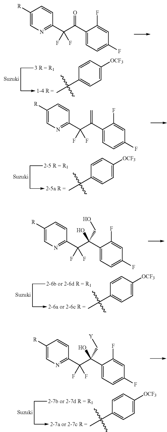
Scheme 3. Synthesis of 1 via Asymmetric Dihydroxylation Method
