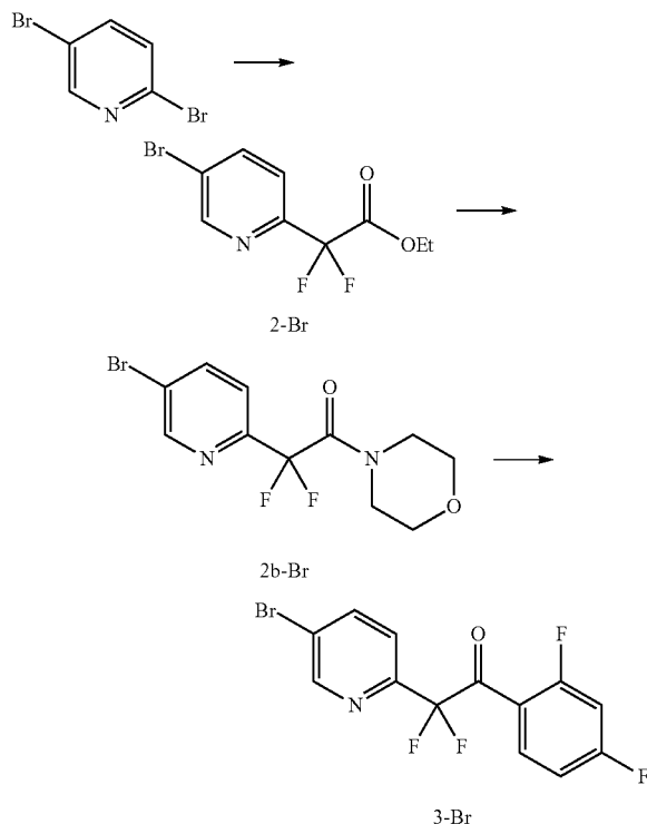
Scheme 1. Synthesis of ketone 3-Br
