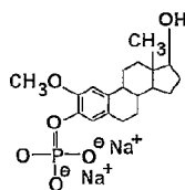
2 - Methoxyestradiol sodium phosphate prodrug
