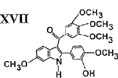
3 - (3',4',5' trimethoxy benzoyl) -2- (4' - methoxy 5' - hydroxy phenyl) -6-methoxy indole
