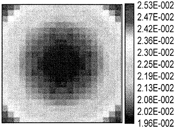
RMS Spot Radius Field Map
