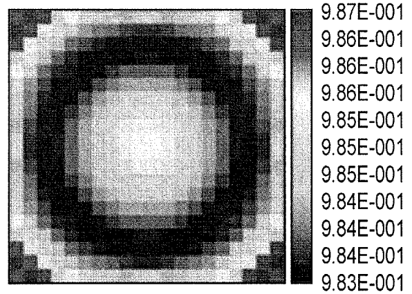
Strehl Ratio field Map
