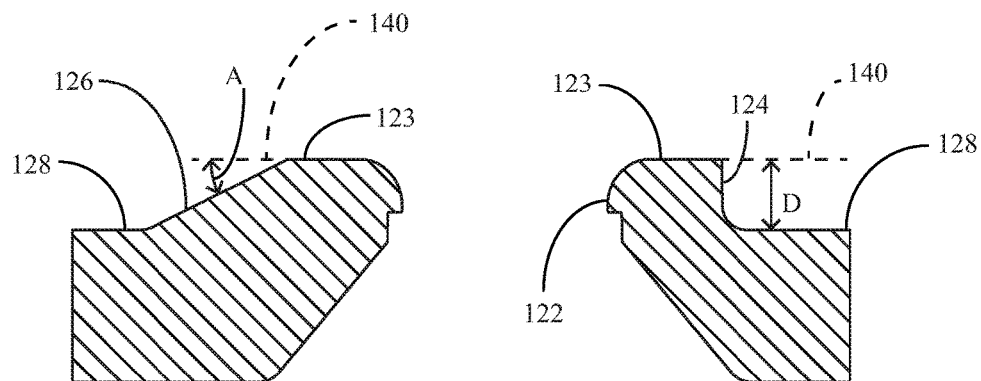
SEC. X-X
