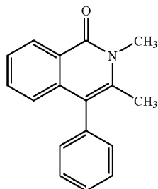
2,3-Dimethyl-4-phenyl-2H-isoquinolin-1-one
