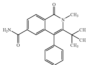
3-tert-butyl-2-methyl-1-oxo-4-phenyl-1,2-dihydroisoquinoline-6-carboxamide
