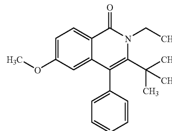
3-tert-butyl-2-ethyl-6-methoxy-4-phenylisoquinolin-1(2H)-one
