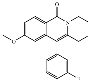
11-(3-fluorophenyl)-9-methoxy-1,2,3,4-tetrahydro-6H-pyrido[1,2-b]isoquinolin-6-one
