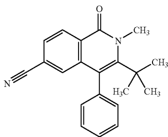
3-tert-butyl-2-methyl-1-oxo-4-phenyl-1,2-dihydroisoquinoline-6-carbonitrile
