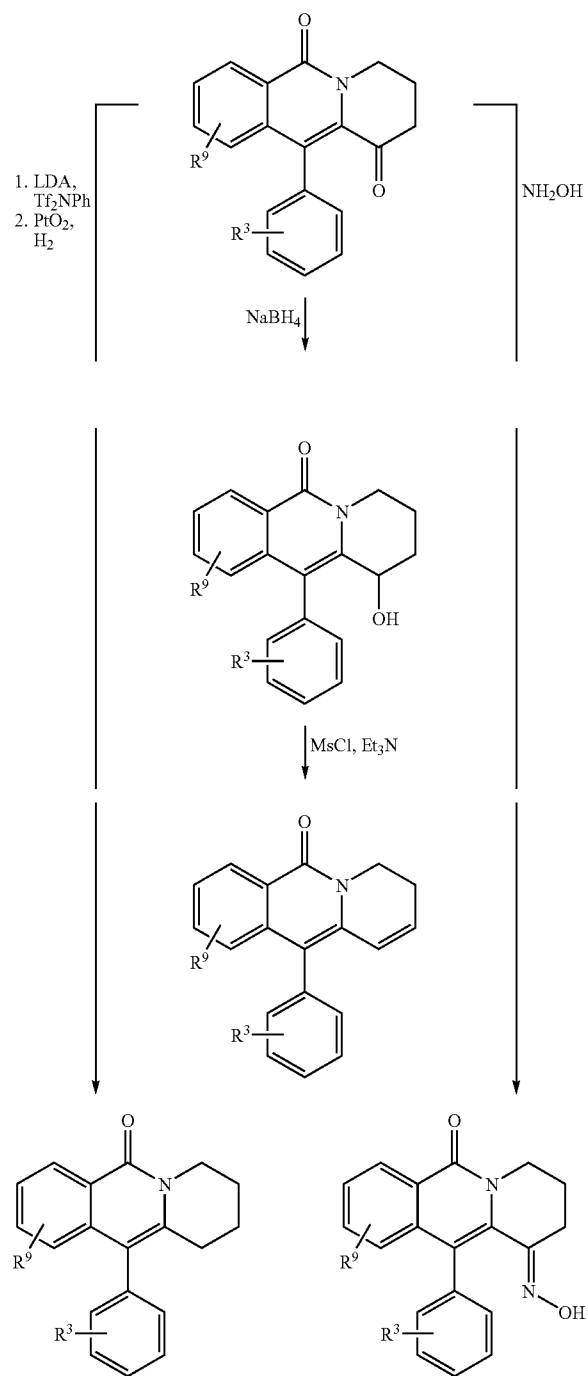
Scheme 2
