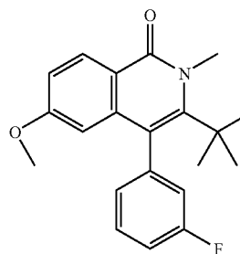
3-tert-butyl-4-(3-fluorophenyl)-6-methoxy-2-methylisoquinolin-1(2H)-one
