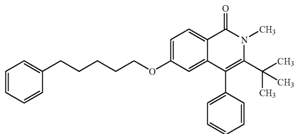
3-tert-butyl-2-methyl-4-phenyl-6-[(5-phenylpentyl)oxy]isoquinolin-1(2H)-one
