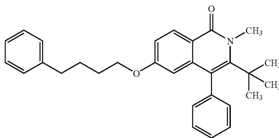
3-tert-butyl-2-methyl-4-phenyl-6-(4-phenylbutoxy)isoquinolin-1(2H)-one
