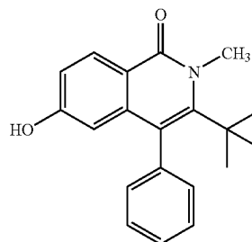
3-tert-Butyl-6-hydroxy-2-methyl-4-phenyl-2H-isoquinolin-1-one
