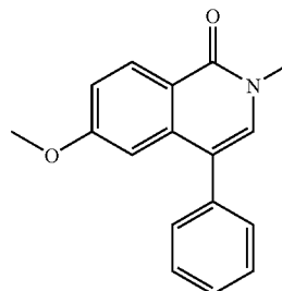
6-methoxy-2-methyl-4-phenylisoquinolin-1(2H)-one
