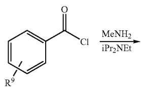
Scheme 3
