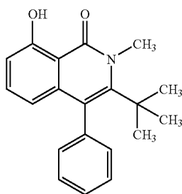
3-tert-butyl-8-hydroxy-2-methyl-4-phenylisoquinolin-1(2H)-one
