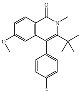
3-tert-butyl-4-(4-fluorophenyl)-6-methoxy-2-methylisoquinolin-1(2H)-one
