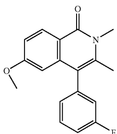
4-(3-fluorophenyl)-6-methoxy-2,3-dimethylisoquinolin-1(2H)-one
