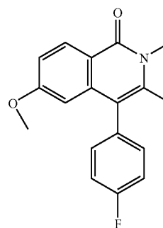
4-(4-fluorophenyl)-6-methoxy-2,3-dimethylisoquinolin-1(2H)-one
