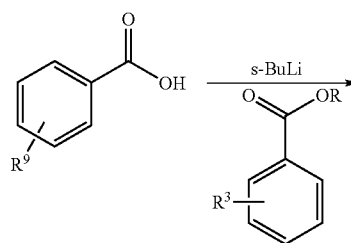
Scheme 1
