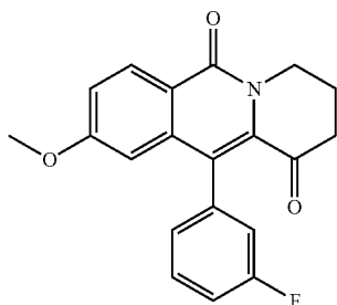
11-(3-fluorophenyl)-9-methoxy-3,4-dihydro-2H-pyrido[1,2-b]isoquinoline-1,6-dione
