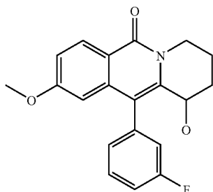
11-(3-fluorophenyl)-1-hydroxy-9-methoxy-1,2,3,4-tetrahydro-6H-pyrido[1,2-b]isoquinolin-6-one
