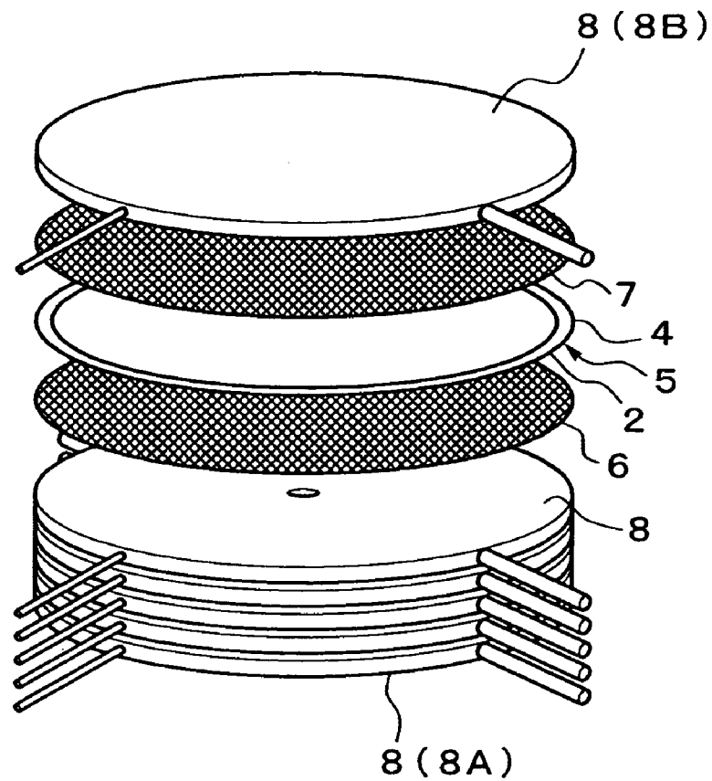
FIG. 7 (PRIOR ART)
