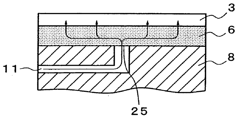
FIG. 8 (PRIOR ART)
