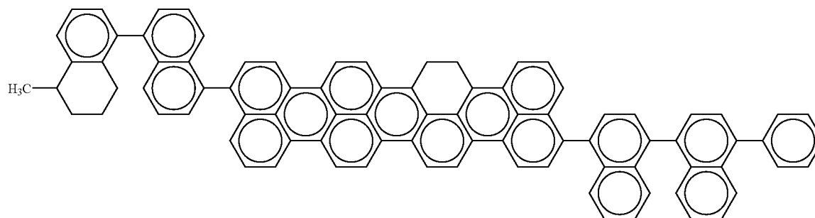
AR, synthesized pitch
