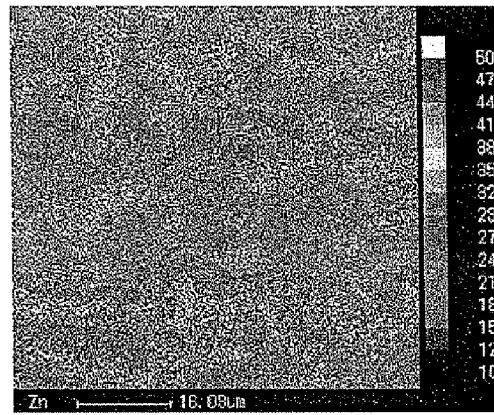
Zn SPECTRUM
