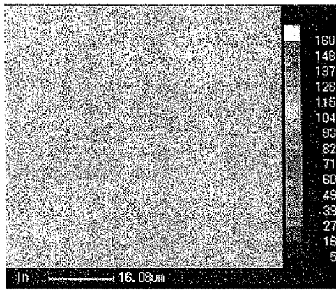
In SPECTRUM
