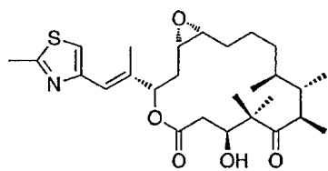
Epothilone A
