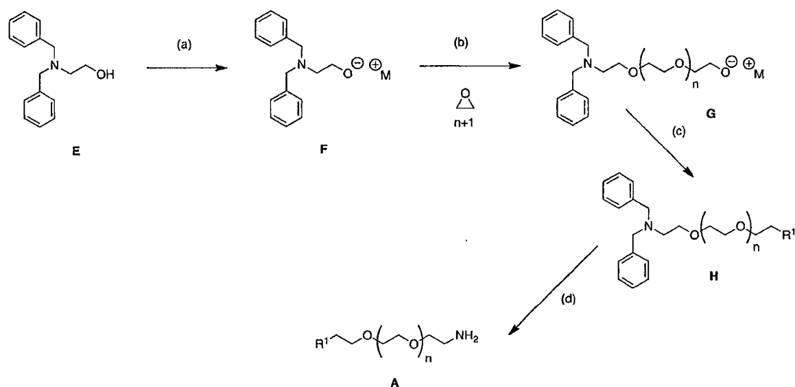
Scheme 4
