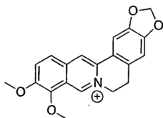
Berberine
