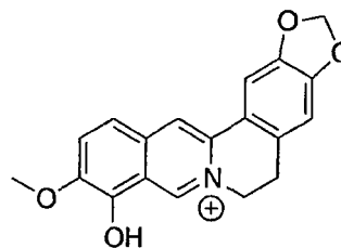
Berberrubine
