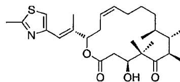
Epothilone C
