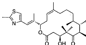
Epothilone D
