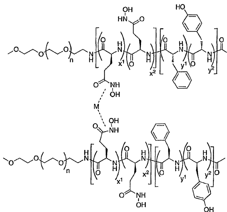
IX
