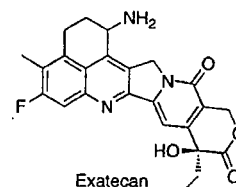
Exatecan
