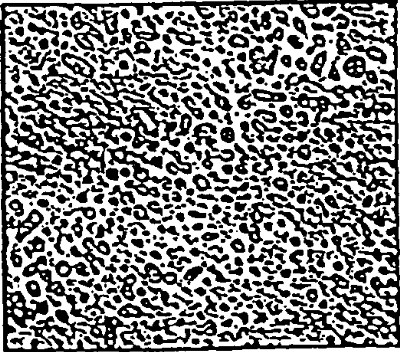
BCTP-Treated Spores
