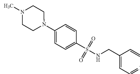
4-(4-methylpiperazin-1-yl)-N-(pyridin-4-ylmethyl) benzenesulfonamide
