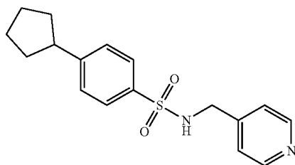
4-cyclopentyl-N-(pyridin-4-ylmethyl)benzenesulfonamide
