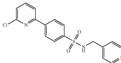
4-(6-chloropyridin-2-yl)-N-(pyridin-4-ylmethyl)benzenesulfonamide
