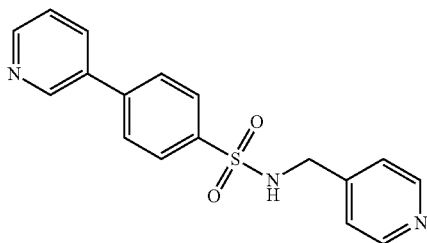
4-(pyridin-3-yl)-N-(pyridin-4-ylmethyl)benzenesulfonamide
