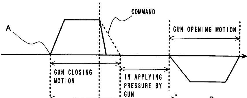
FIG. 3 a VELOCITY OF SERVO GUN AXIS MOTOR
