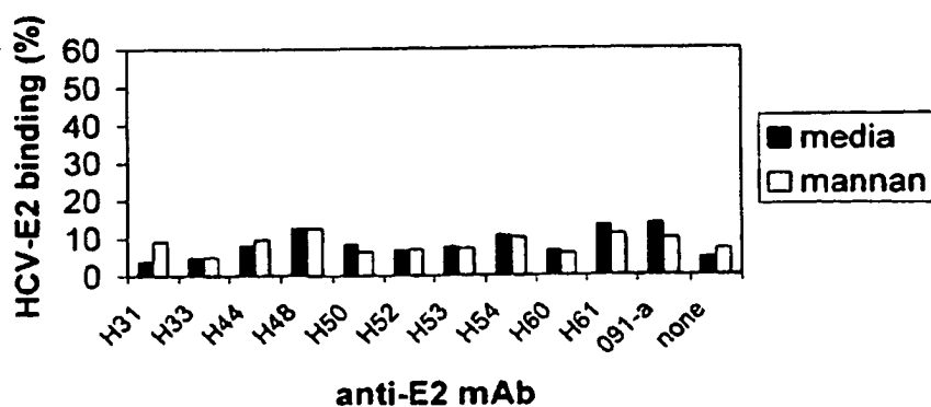
Figure 5. DC-SIGN and DC-SIGNR transfectants bind HCV-E2. (A) HeLa-DC-SIGN, (B) HeLa-DC-SIGNR and (C) parental HeLa cells were allowed to bind to HCV-E2-coated beads that were prepared by conjugation with a panel of anti-E2 mAbs. Adhesion was quantified by FACS analysis, and was blocked by mannan (20ug/ml), and one representative experiment out of three is shown.
