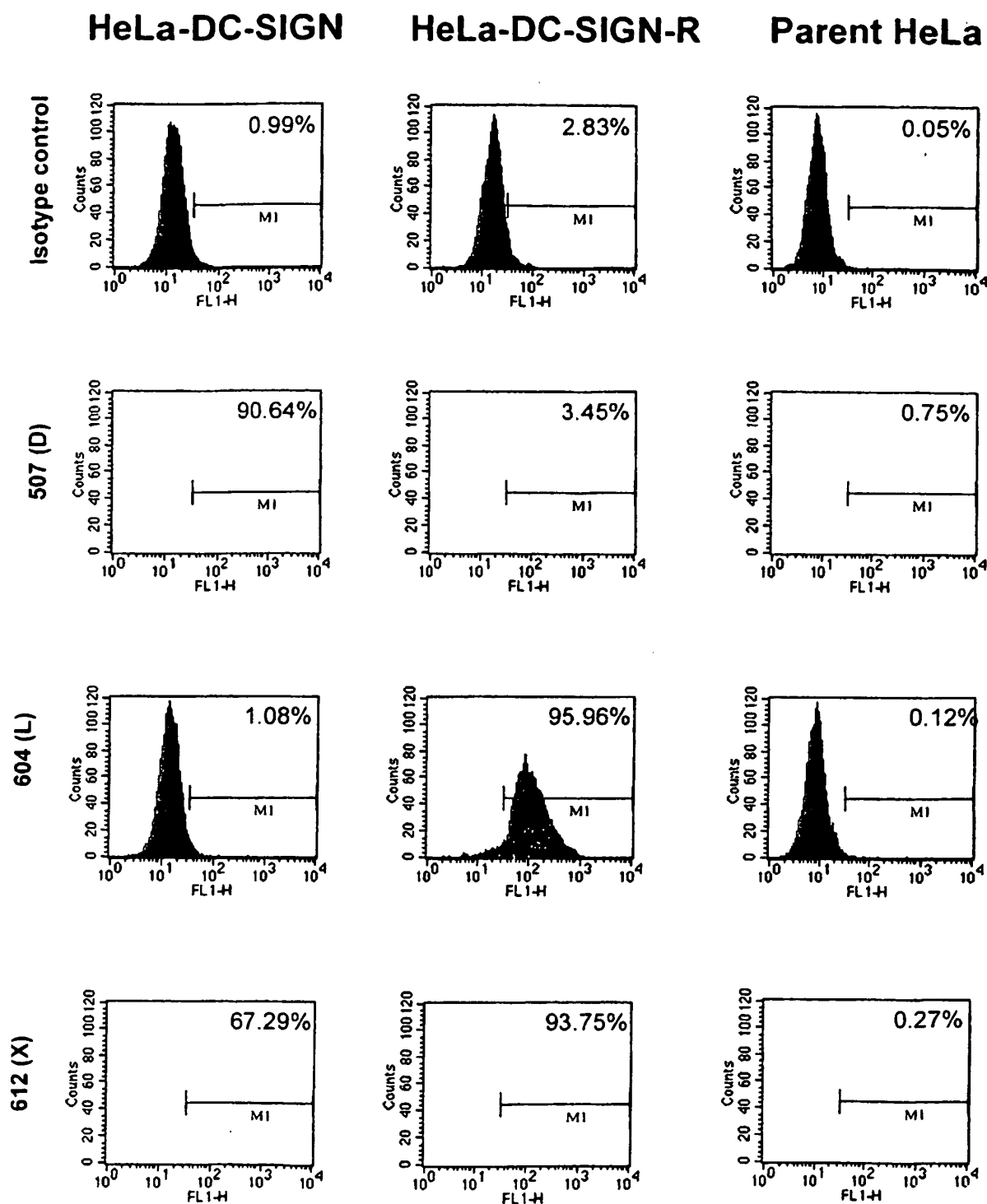
Figure 4. Characterization of HeLa-DC-SIGN and HeLa-DC-SIGN-R cell lines using antibodies specific for DC-SIGN (507(D)), DC-SIGN-R (604(L)) or both molecules (612(X)).
