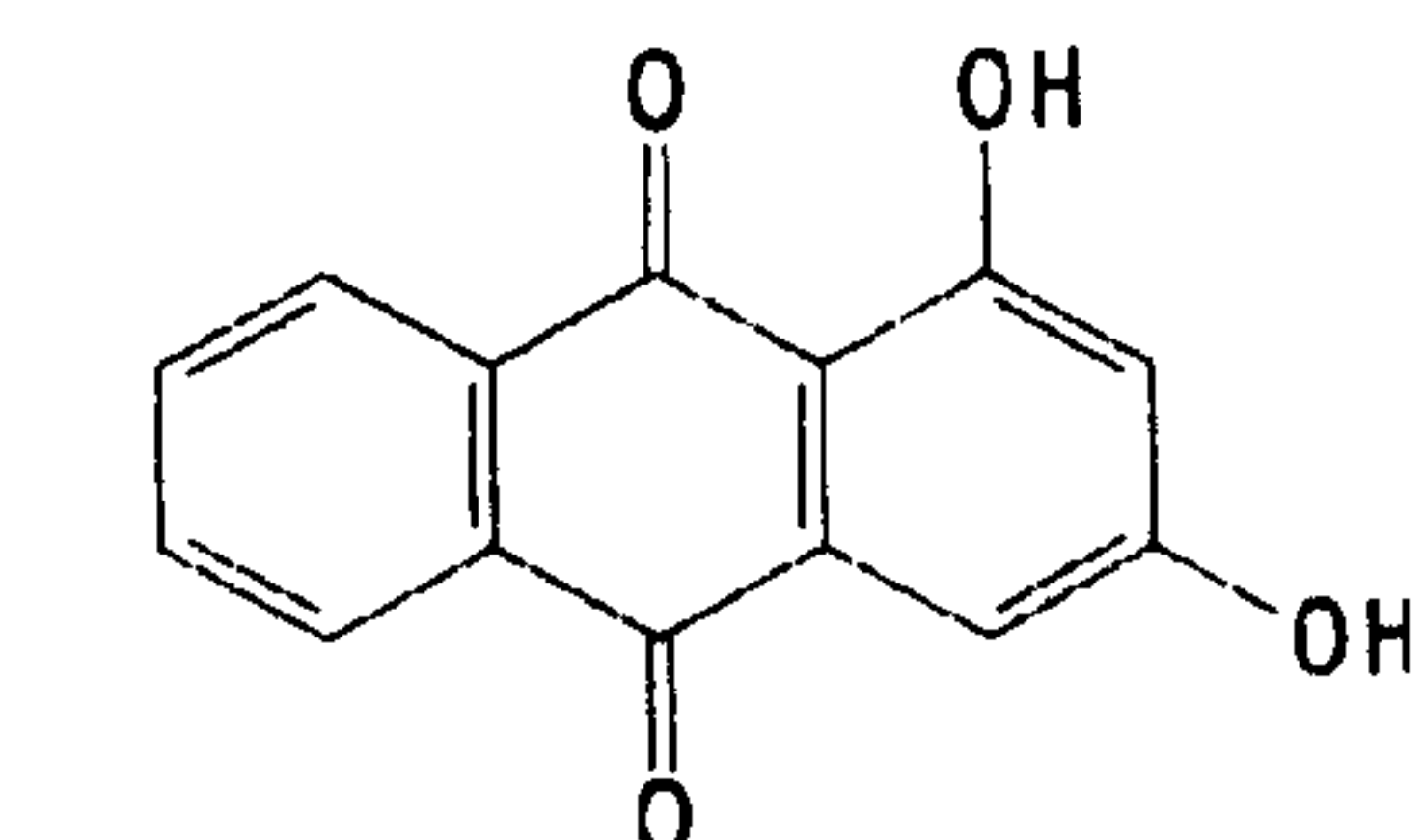
1,3-dihydroxy anthraquinone
