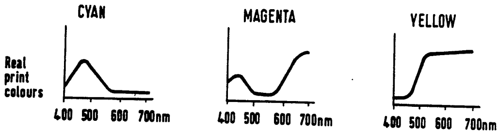
Spectral curve for ideal and real print colours.
