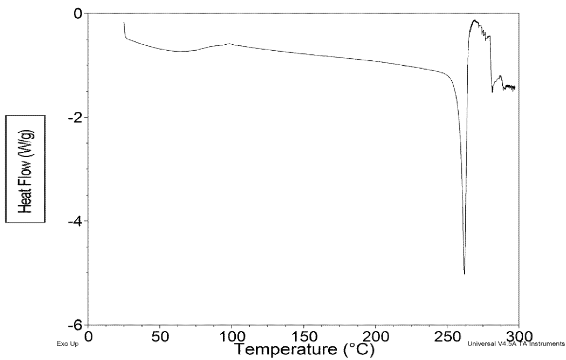
Figure 19: DSC Thermogram N-(2-{2-dimethylaminoethyl-methylamino}-4-methoxy-5-{[4-(1-methylindol-3-yl)pyrimidin-2-yl]amino}phenyl)prop-2-enamide Mesylate salt - Form A
