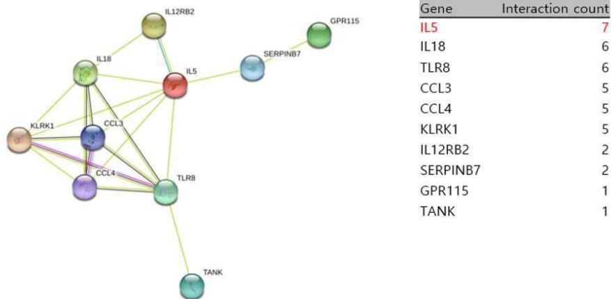
Cluster 2
