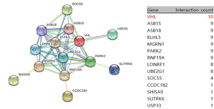
Cluster 1
