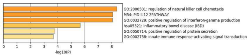
Cluster 2
