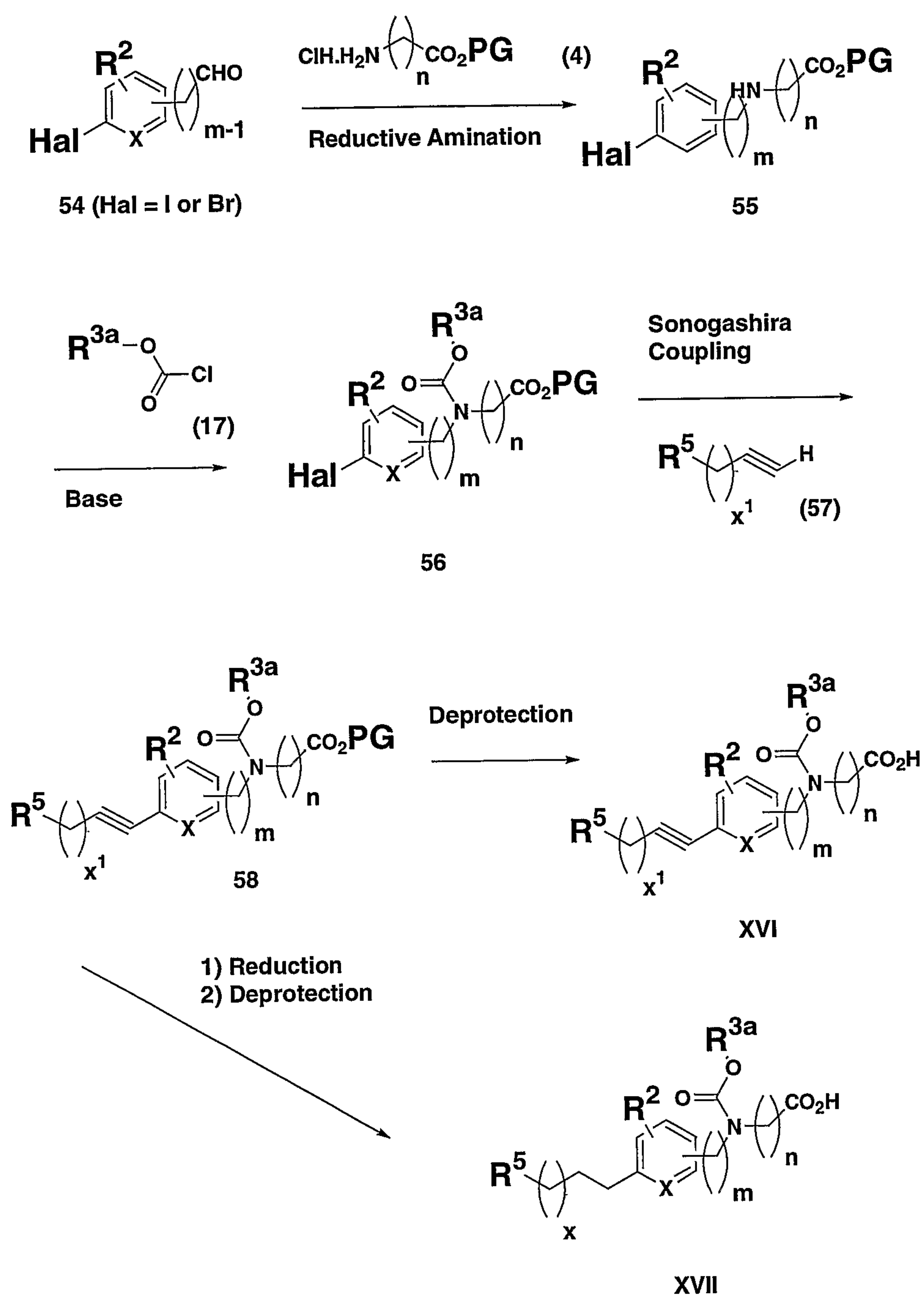
Scheme 17
