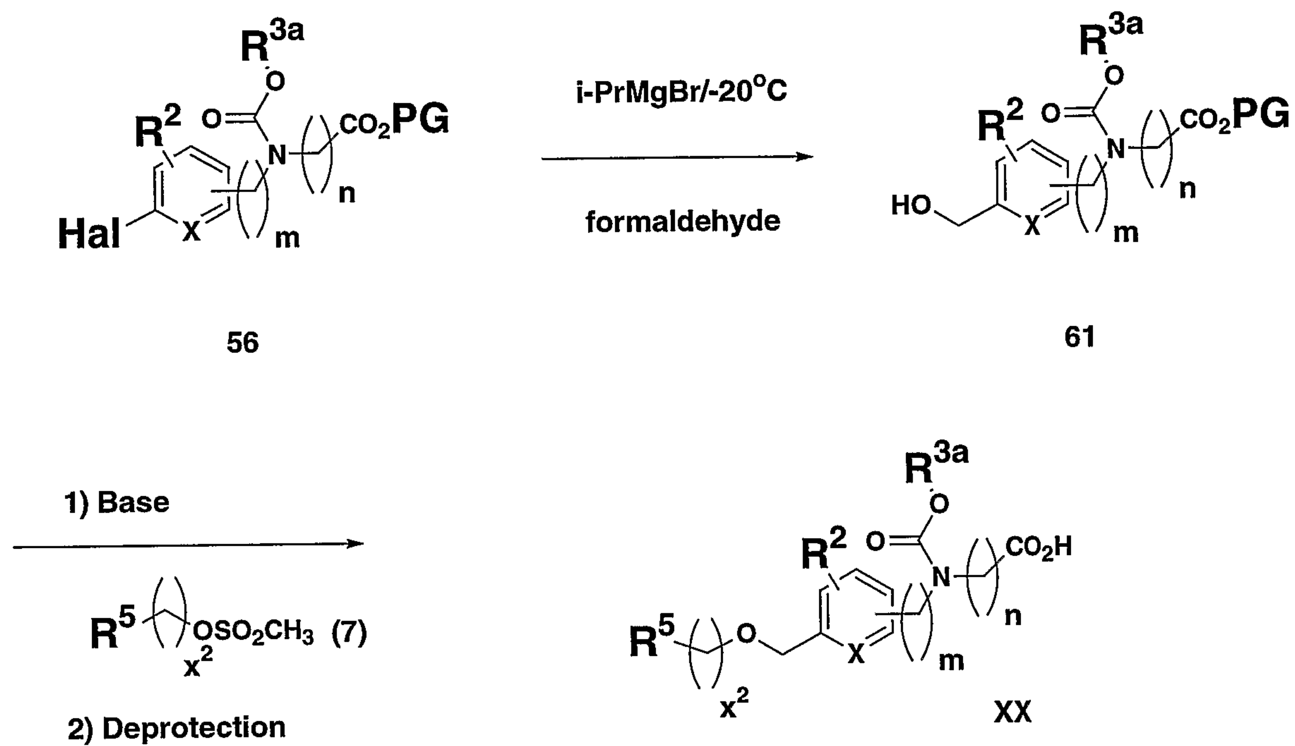
Scheme 20
