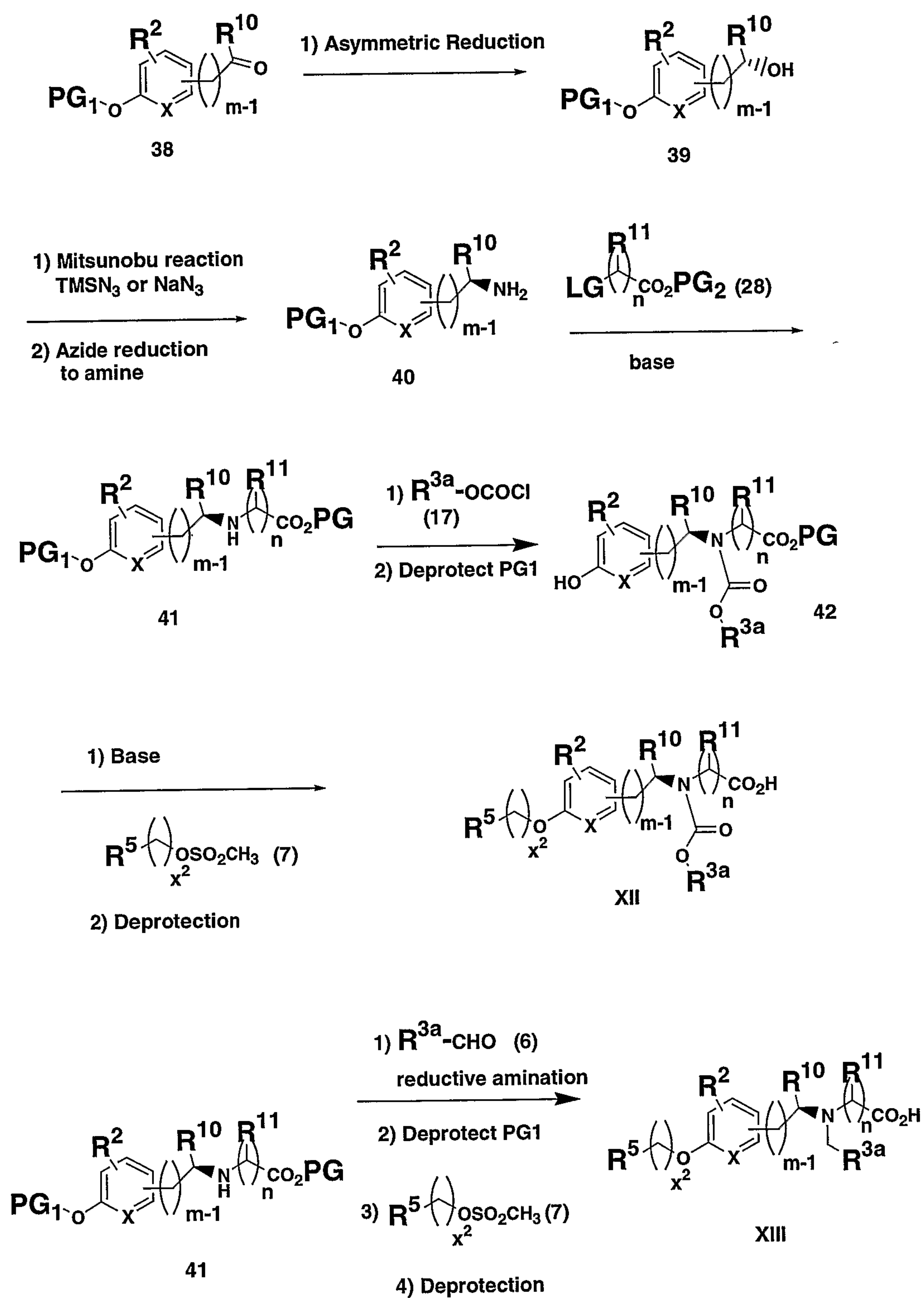
Scheme 14
