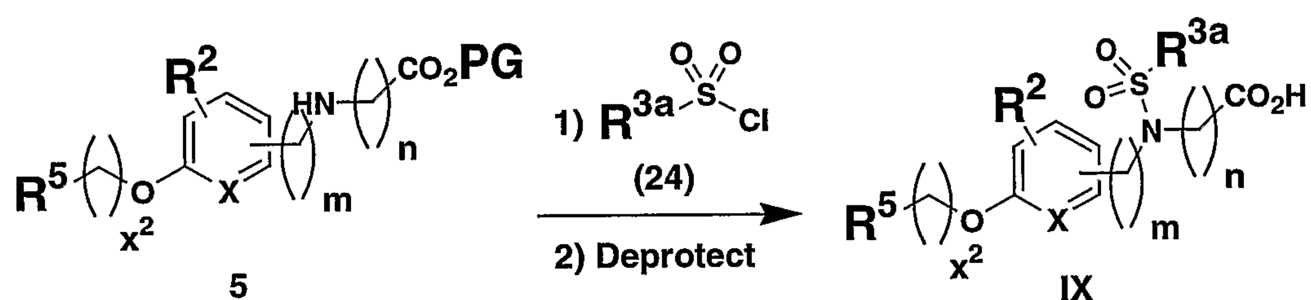
Scheme 10
