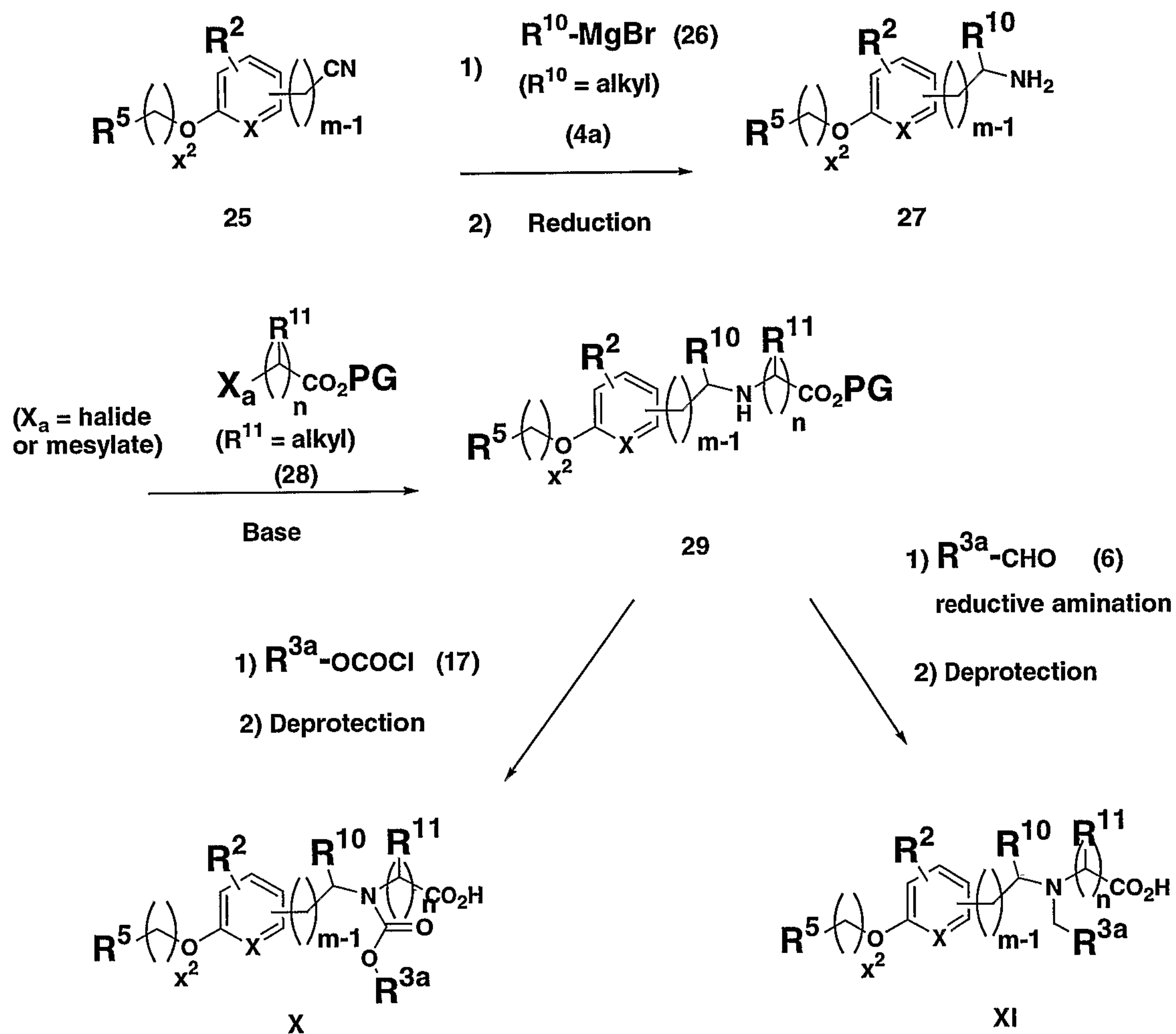
Scheme 11
