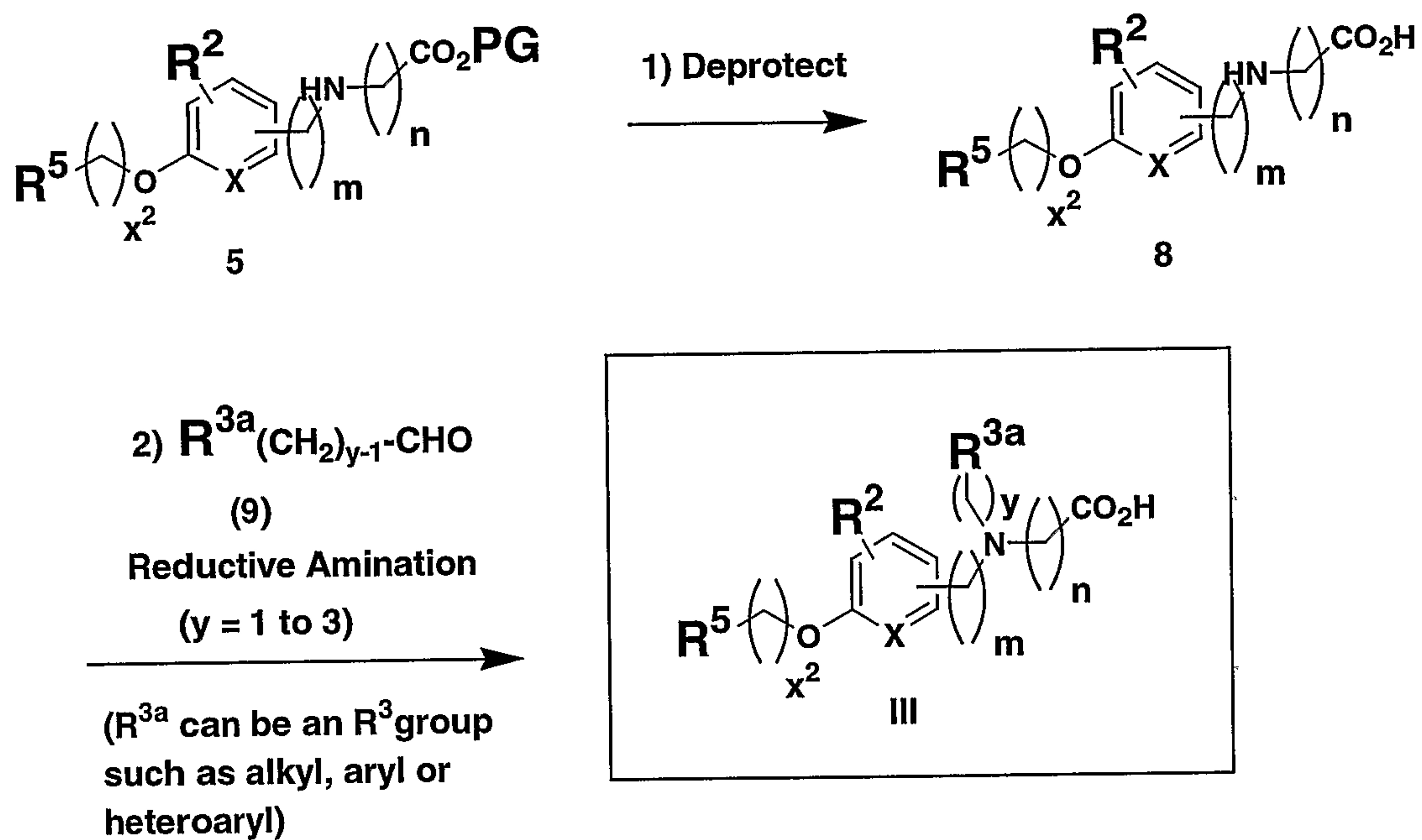
Scheme 2
