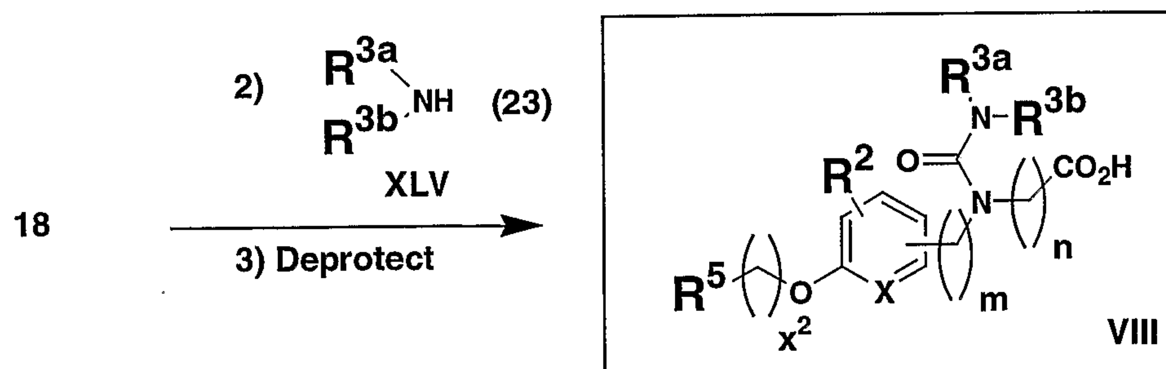
Scheme 9
