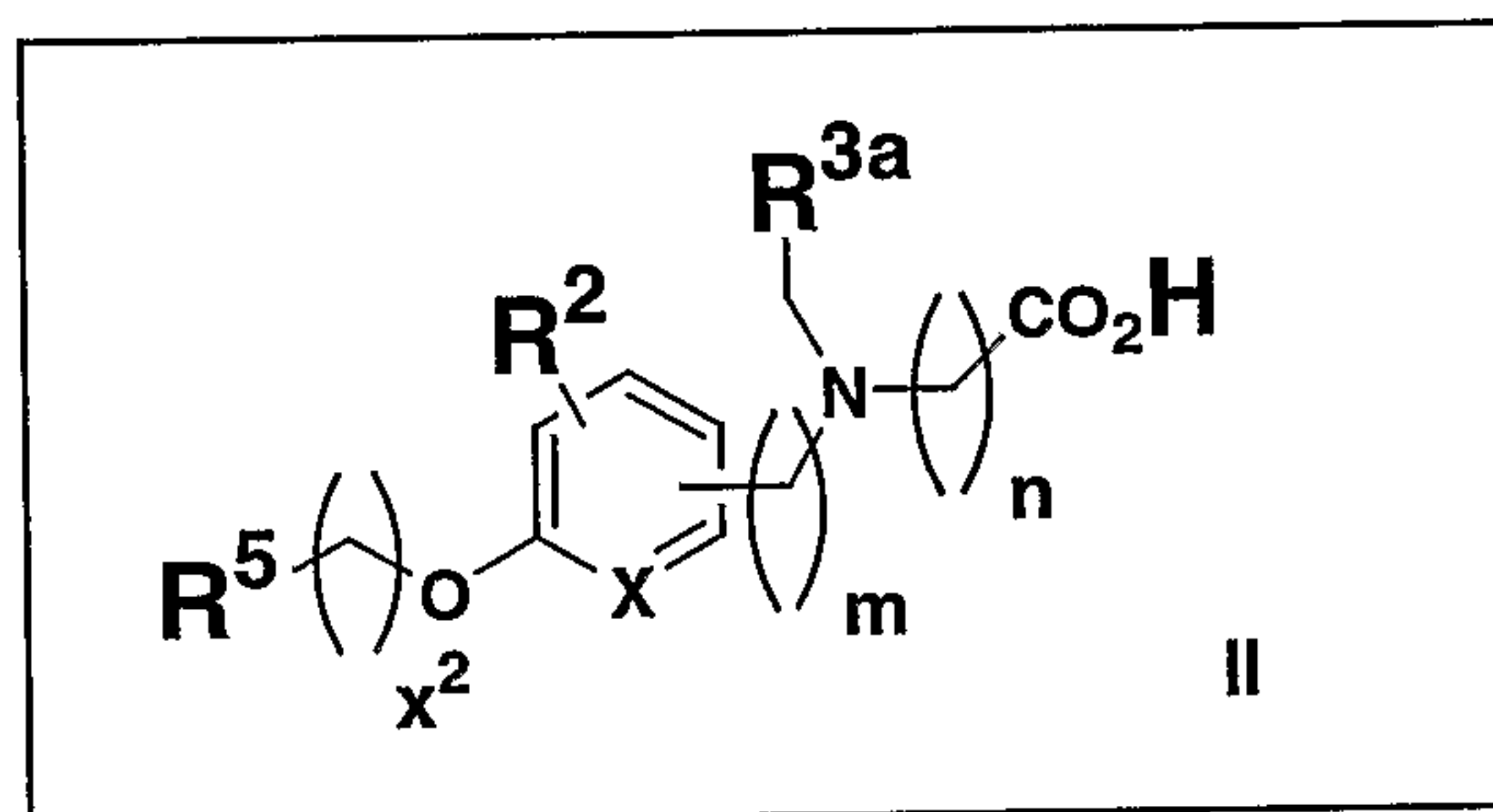
Scheme 1
