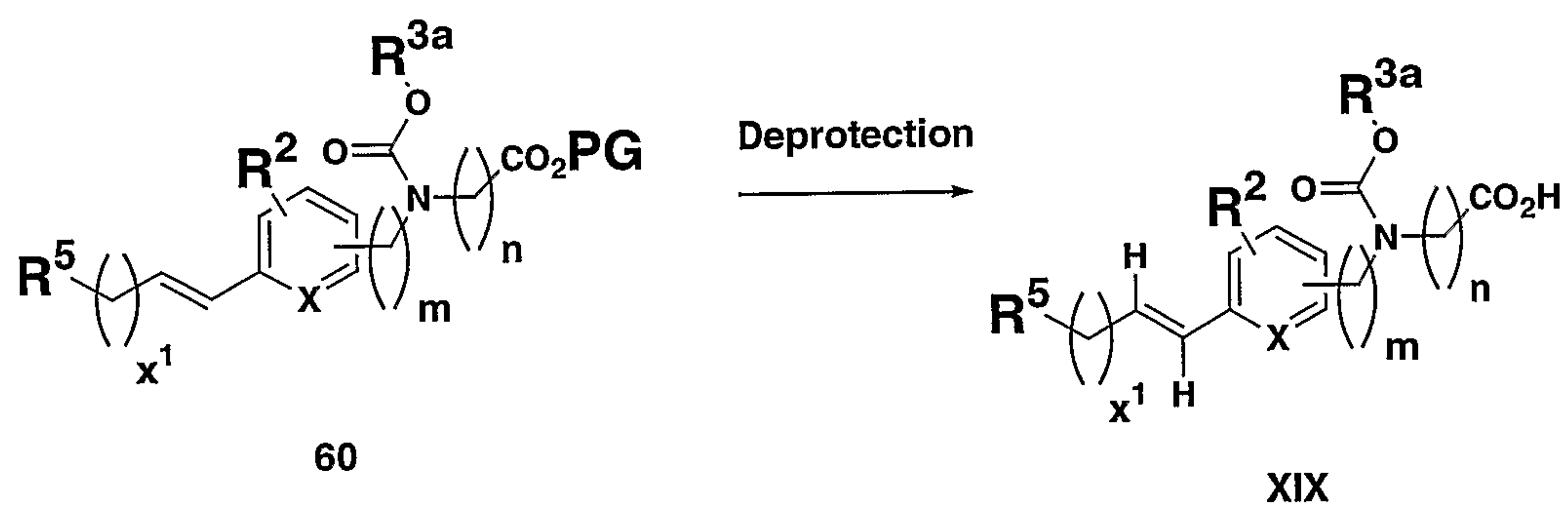
Scheme 19
