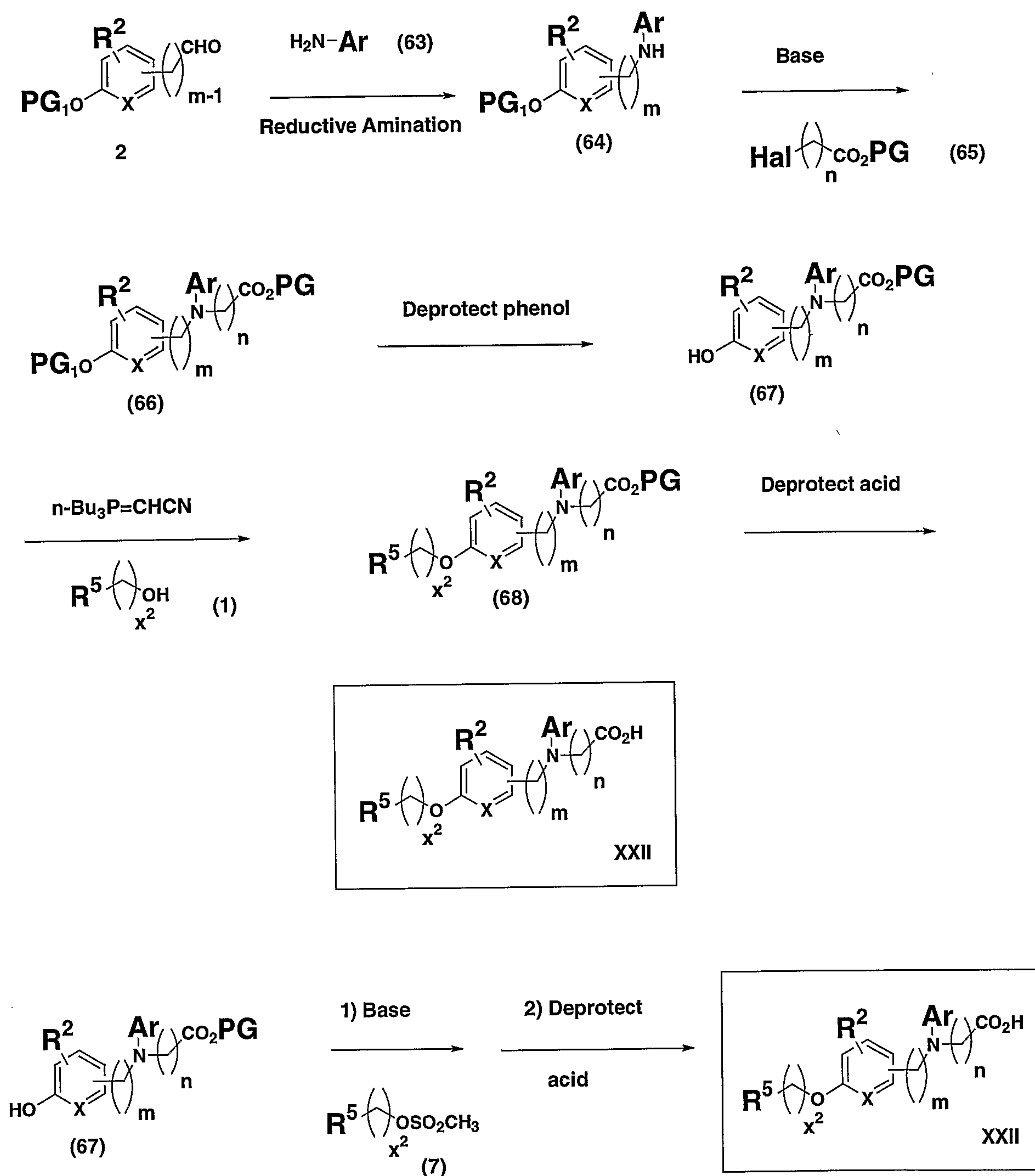
Scheme 22
