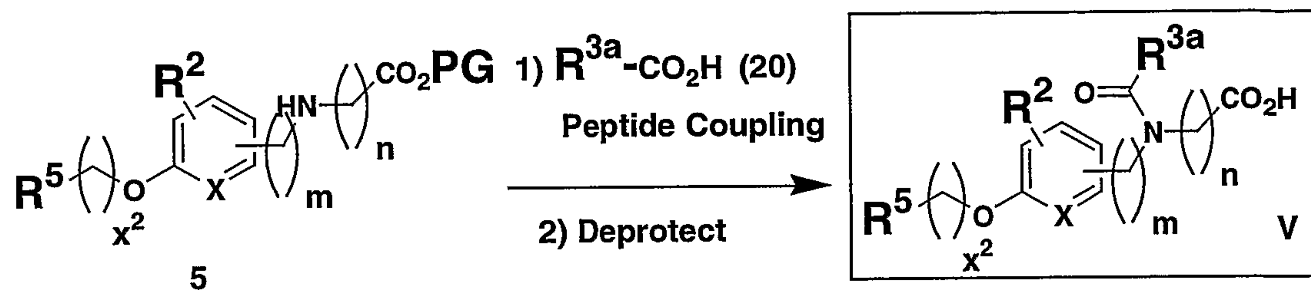
Scheme 7
