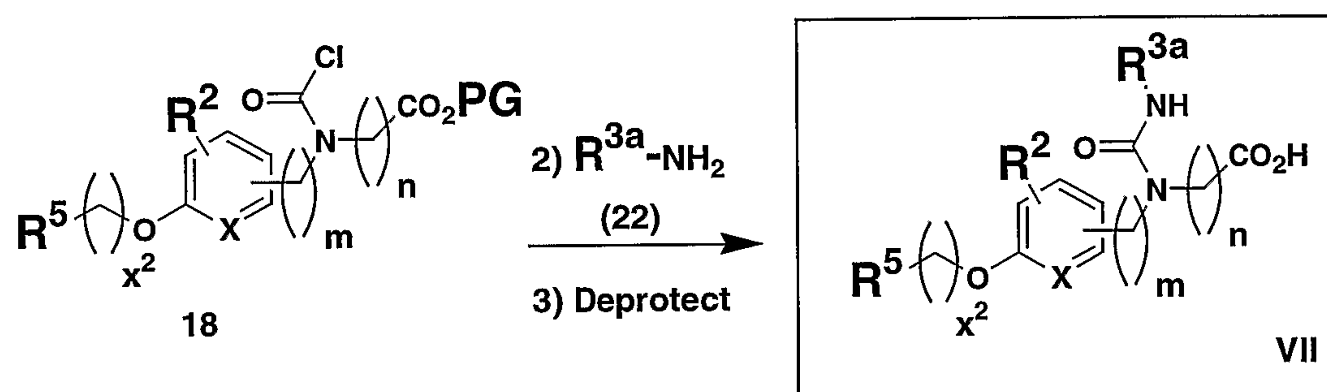
Scheme 8
