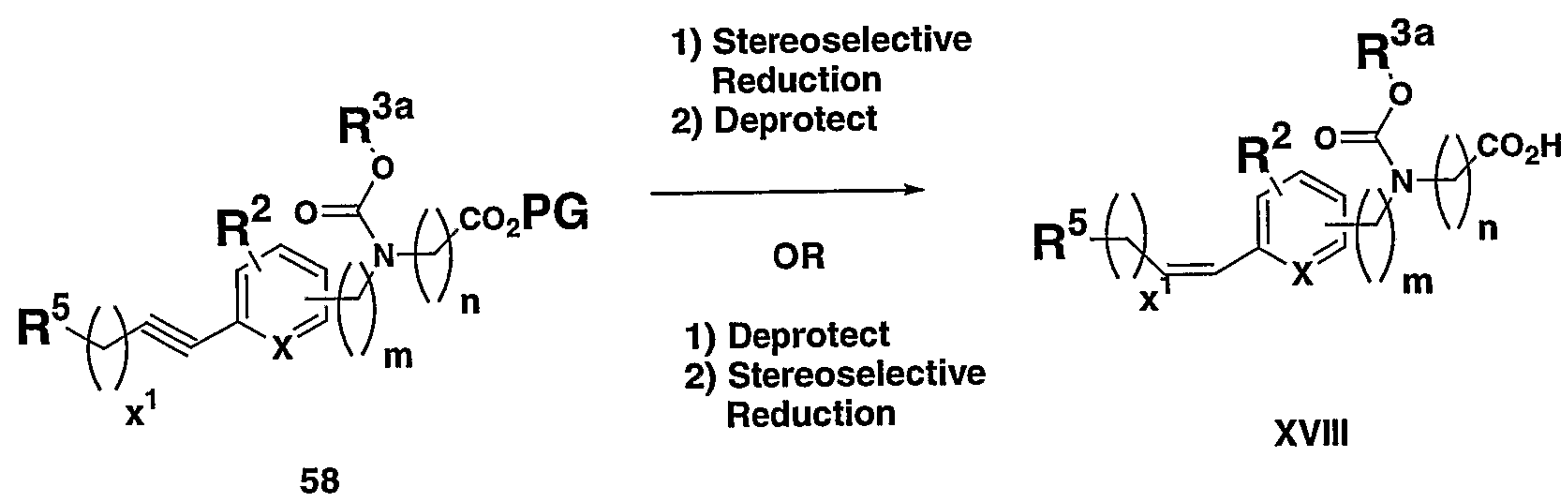
Scheme 18
