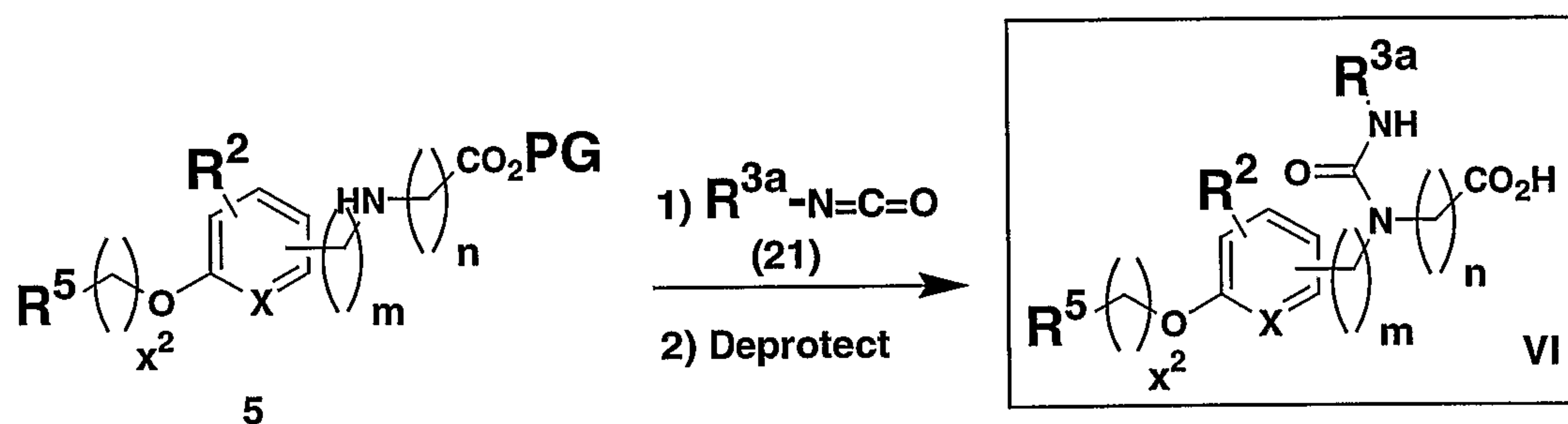
Scheme 7
