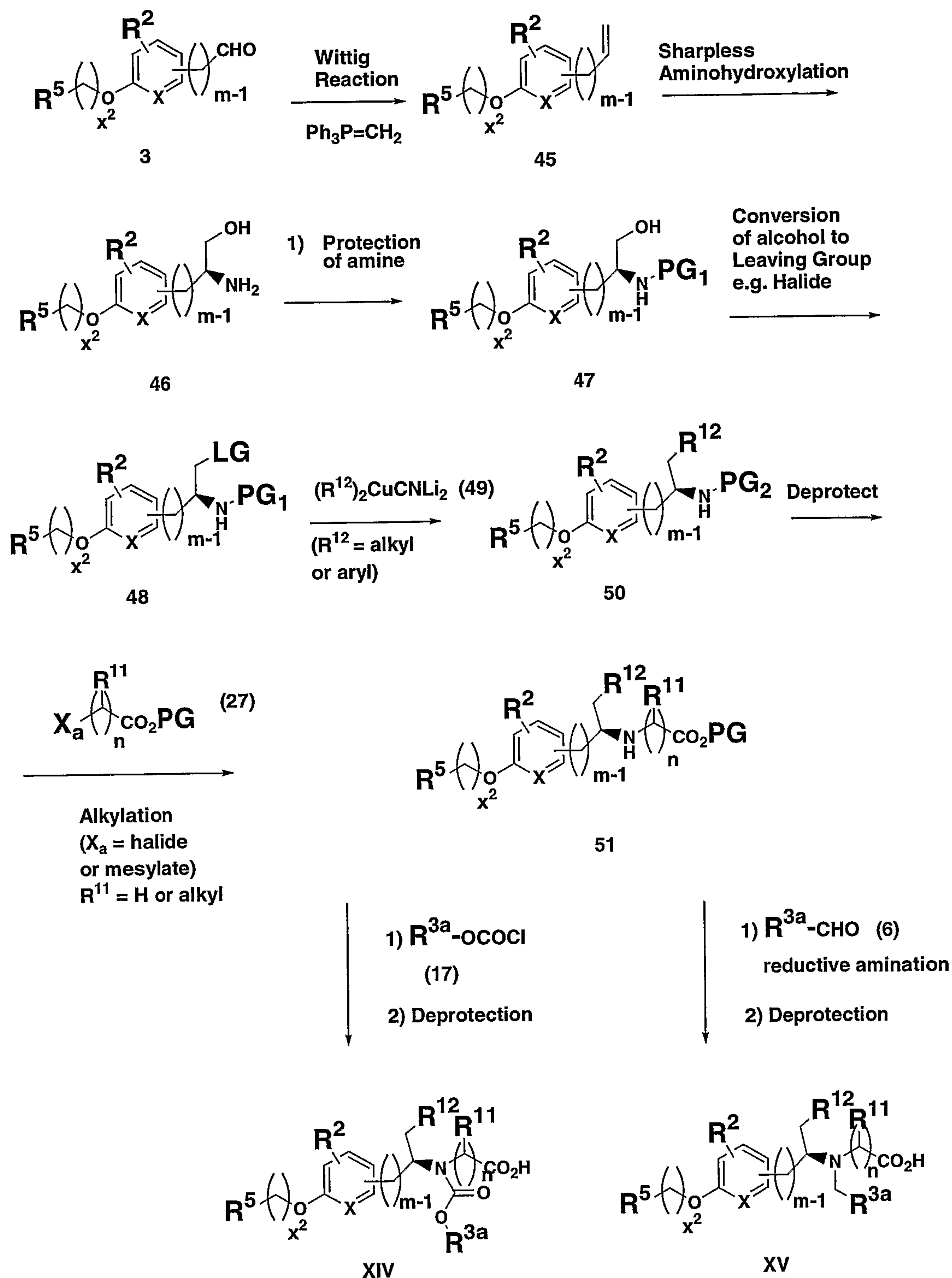
Scheme 16
