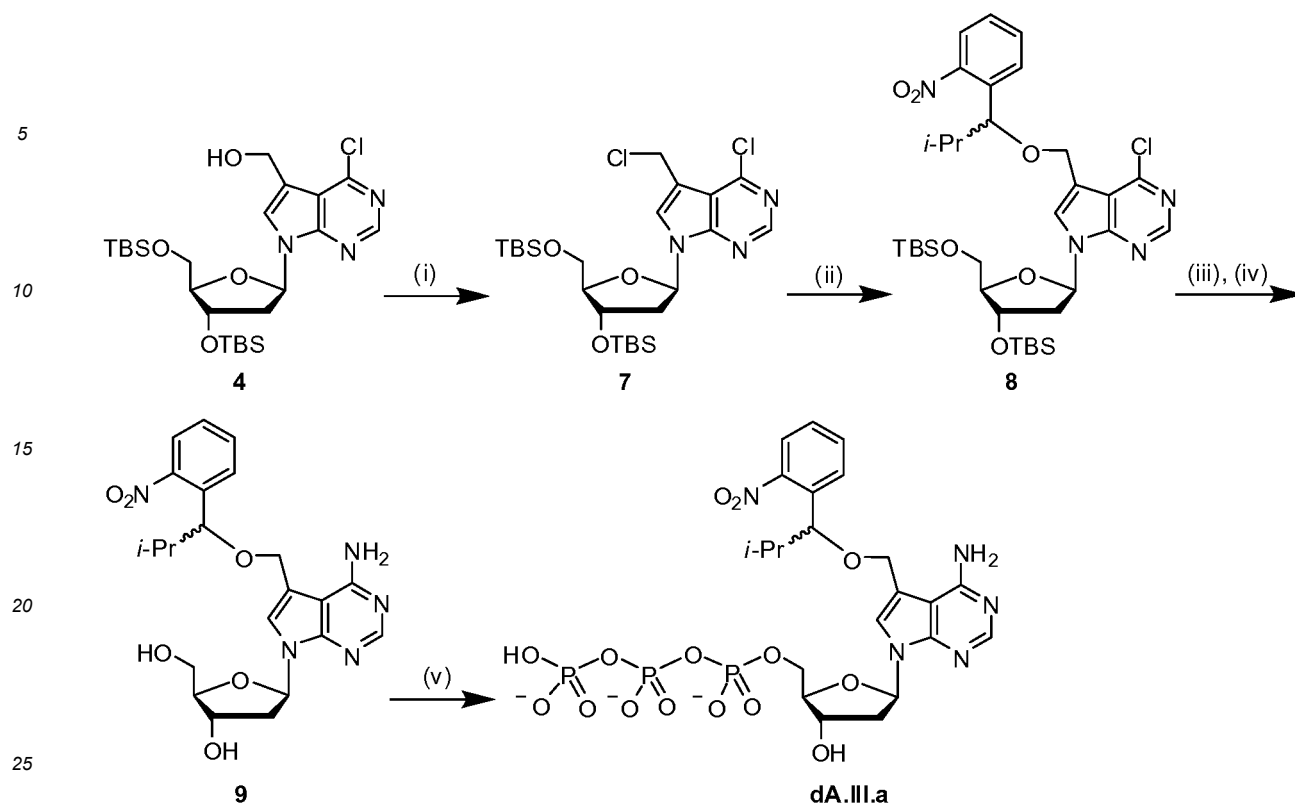
Scheme S7. Synthesis of 7-[1-(2-nitrophenyl)-2-methyl-propyloxy]methyl-7-deaza-2'-deoxyadenosine-5'-triphosphate. Reagents and conditions: (i) TsCl, DMAP, CH 2 Cl 2 , room temperature, 39%; (ii) racemic ( R/S )-1-(2-nitrophenyl)-2-methyl-propanol, neat, 105°C, 54%; (iii) n -Bu 4 NF, THF, 0°C to room temperature; (iv) NH 3 , 1,4-dioxane/MeOH, 100°C, 76% for two steps; (v) POCl 3 , (MeO) 3 PO, minus 40°C to 0°C; ( n -Bu 3 NH) 2 H 2 P 2 O 7 , n -Bu 3 N, DMF; 1 M HNEt 3 HCO 3 .
