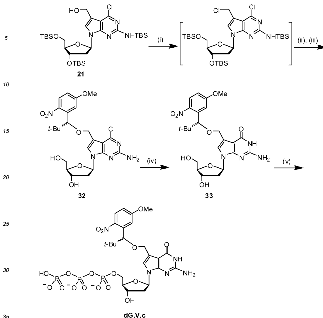
Scheme S16. Synthesis of 7-[1-(5-methoxy-2-nitrophenyl)-2,2-dimethyl-propyloxy]methyl-7-deaza-2'-deoxyguanosine-5'-triphosphate. Reagents and conditions: (i) MsCl, DMAP, CH 2 Cl 2 , 0°C; (ii) racemic ( R/S )-1-(5-methoxy-2-nitrophenyl)-2,2-dimethyl-1-propanol, 115°C; (iii) n -Bu 4 NF, THF, room temperature, 24% for three steps; (iv) syn-pyridine-2-aldoxime, 1,1,3,3-tetramethyl guanidine, 1,4-dioxane/DMF, 70°C, 57%; (v) POCl 3 , proton sponge, (MeO) 3 PO, 0°C; ( n -Bu 3 NH) 2 H 2 P 2 O 7 , n -Bu 3 N, DMF; 1 M HNEt 3 HCO 3 .
