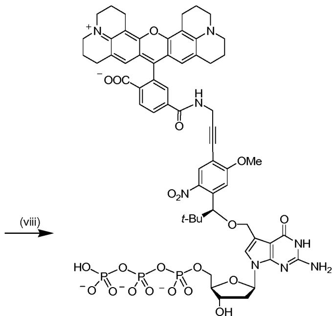
Scheme 4c. (viii) 6-ROX NHS, 0.1 M Na 2 CO 3 /NaHCO 3 buffer (pH 9.2).
