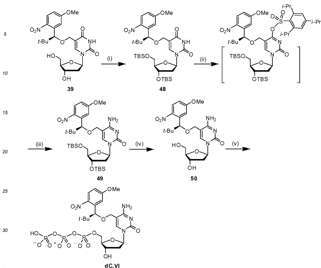
Scheme S22. Synthesis of 5-[(S)-1-(5-methoxy-2-nitrophenyl)-2,2-dimethyl-propyloxy]methyl-2'-deoxycytidine-5'-triphosphate. Reagents and conditions: (i) TBSCl, imidazole, DMF, room temperature, 70%; (ii) 2,4,6-triisopropylbenzenesulfonyl chloride, DMAP, Et 3 N, CH 2 Cl 2 , room temperature; (iii) NH 3 , 1,4-dioxane, 90°C, 65% for two steps; (iv) n -Bu 4 NF, THF, room temperature, 82%; (v) POCl 3 , proton sponge, (MeO) 3 PO, 0°C; ( n -Bu 3 NH) 2 H 2 P 2 O 7 , n -Bu 3 N, DMF; 1 M HNET 3 HCO 3 .
