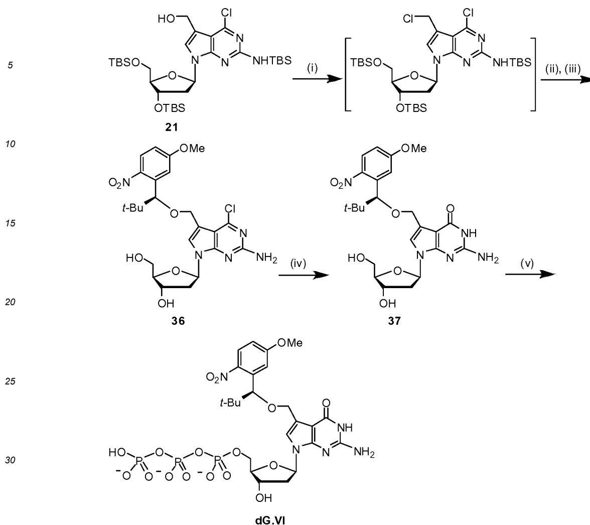
Scheme S18. Synthesis of 7-[(S)-1-(5-methoxy-2-nitrophenyl)-2,2-dimethyl-propyloxy]methyl-7-deaza- 2'-deoxyguanosine-5'-triphosphate. Reagents and conditions: (i) MsCl, DMAP, CH 2 Cl 2 , 0°C; (ii) (S)-1-(5-methoxy-2-nitrophenyl)-2,2-dimethyl-1-propanol, 115°C; (iii) n -Bu 4 NF, THF, room temperature, 27% for three steps; (iv) syn-pyridine-2-aldoxime, 1,1,3,3-tetramethyl guanidine, 1,4-dioxane/DMF, 70°C, 76%; (v) POCl 3 , proton sponge, (MeO) 3 PO, 0°C; ( n -Bu 3 NH) 2 H 2 P 2 O 7 , n -Bu 3 N, DMF; 1 M HNEt 3 HCO 3 .
