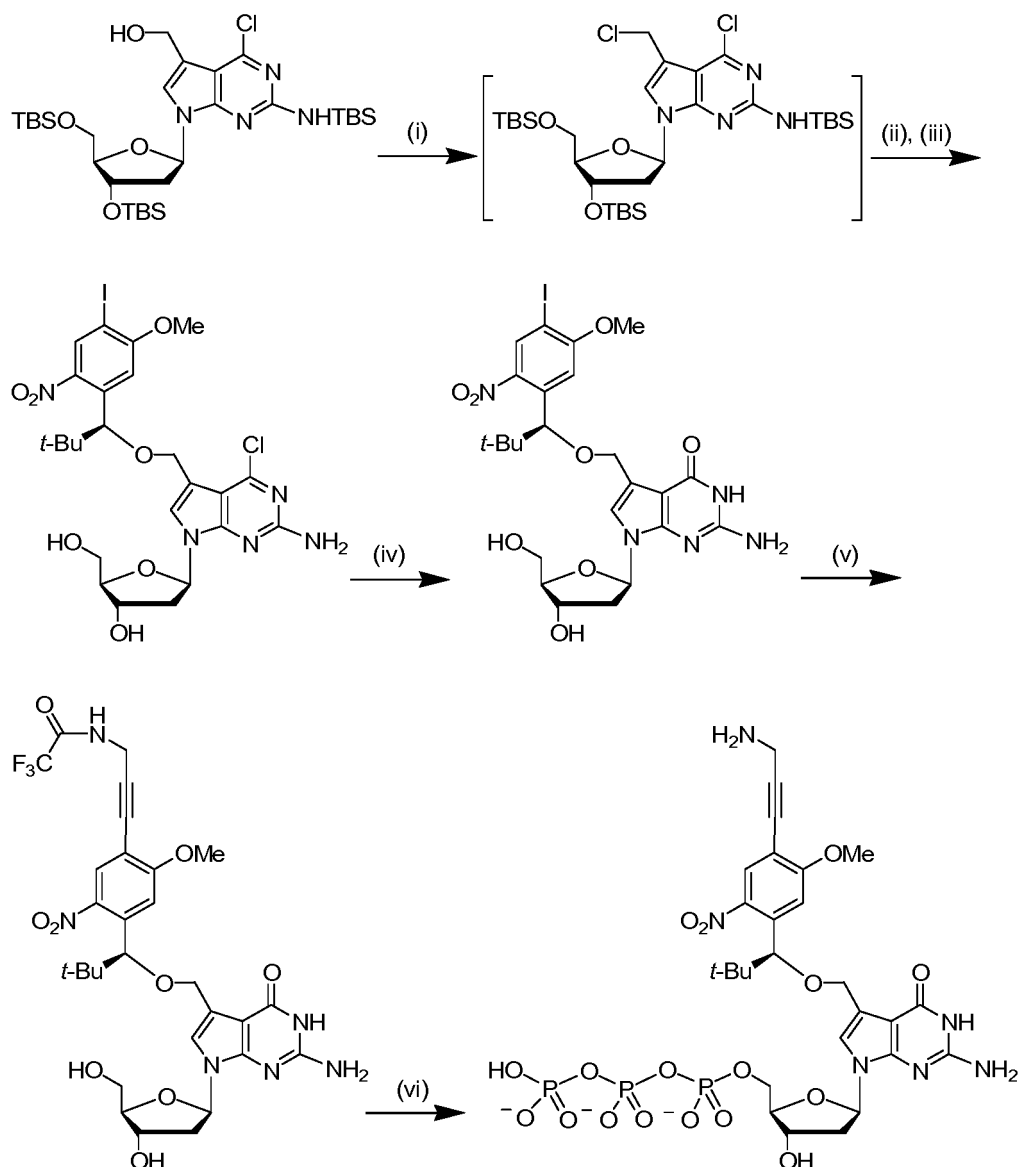
Scheme 4a. Synthesis of dye labeled 7-[(S)-1-(5-methoxy-2-nitrophenyl)-2,2-dimethyl-propyloxy]methyl-7-deaza-2'-deoxyguanosine-5'-triphosphate. Reagents and conditions: (i) MsCl, DMAP, CH 2 Cl 2 , 0°C; (ii) (S)-1-(4-iodo-5-methoxy-2-nitrophenyl)-2,2-dimethyl-1-propanol, 115°C; (iii) n-Bu 4 NF, THF, room temperature; (iv) syn-pyridine-2-aldoxime, 1,1,3,3-tetramethyl guanidine, 1,4-dioxane/DMF, 70°C; (v) N-propargyltrifluoroacetamide, Pd(PPh 3 ) 4 (0), CuI, Et 3 N, DMF; (vi) POCl 3 , proton sponge, (MeO) 3 PO, 0°C; (n-Bu 3 NH) 2 H 2 P 2 O 7 , n-Bu 3 N, DMF; 1 M HNEt 3 HCO 3 .
