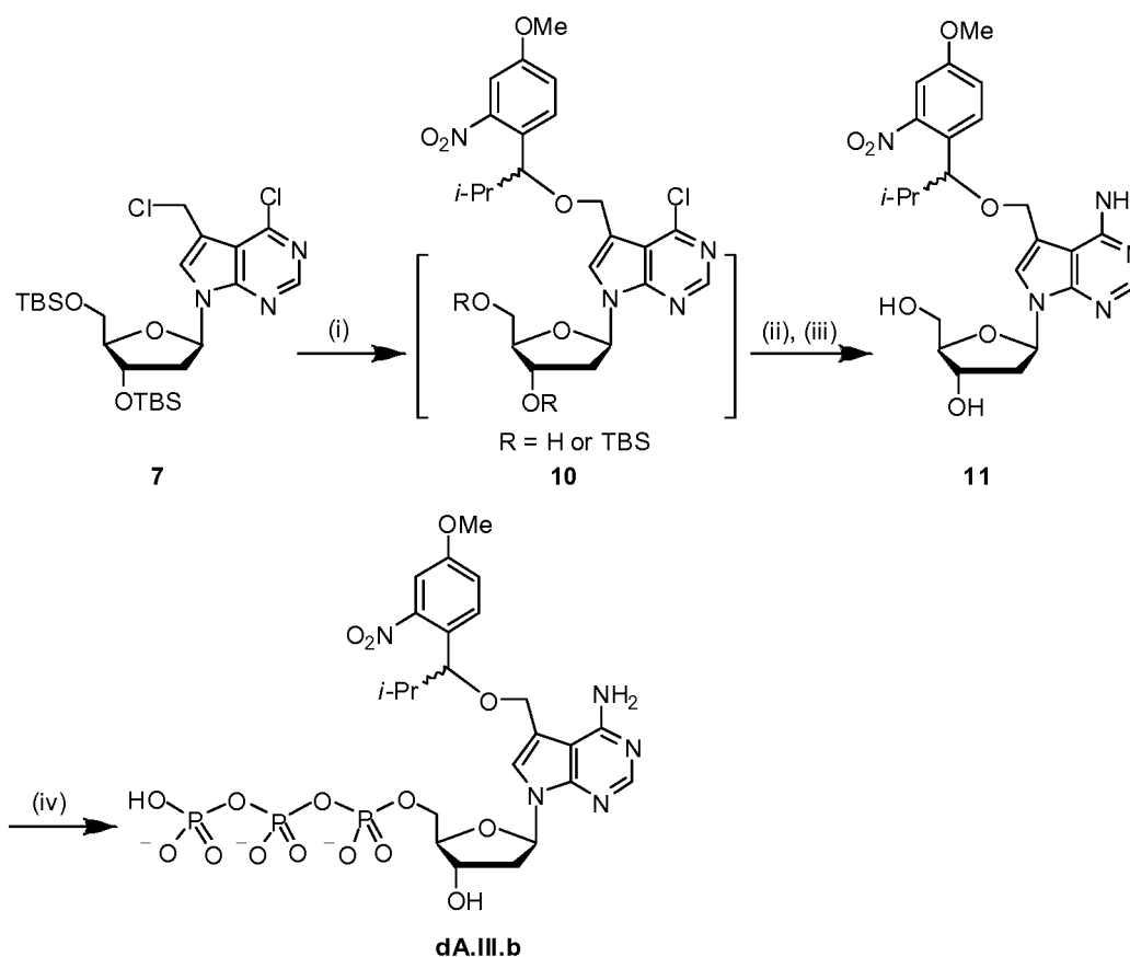
Scheme S8. Synthesis of 7-[1-(4-methoxy-2-nitrophenyl)-2-methyl-propyloxy]methyl-7-deaza-2'-deoxyadenosine-5'-triphosphate. Reagents and conditions: (i) racemic ( R/S )-1-(4-
