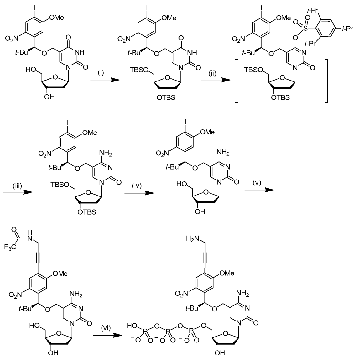
Scheme 5a. Synthesis of dye labeled 5-[(S)-1-(5-methoxy-2-nitrophenyl)-2,2-dimethylpropyloxy]methyl-2'-deoxycytidine-5'-triphosphate. Reagents and conditions: (i) TBSCl, imidazole, DMF, room temperature; (ii) 2,4,6-triisopropylbenzenesulfonyl chloride, DMAP, Et 3 N, CH 2 Cl 2 , room temperature; (iii) NH 3 , 1,4-dioxane, 90°C; (iv) n -Bu 4 NF, THF, room temperature, 82%; (v) N -propargyltrifluoroacetamide, Pd(PPh 3 ) 4 (0), CuI, Et 3 N, DMF; (vi) POCl 3 , proton sponge, (MeO) 3 PO, 0°C; ( n -Bu 3 NH) 2 H 2 P 2 O 7 , n -Bu 3 N, DMF; 1 M HNEt 3 HCO 3 .
