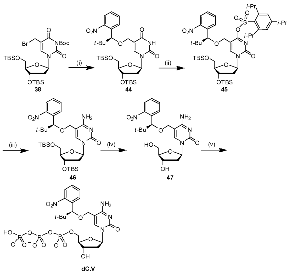
Scheme S21. Synthesis of 5-[(S)-1-(2-nitrophenyl)-2,2-dimethyl-propyloxy]methyl-2'-deoxycytidine-5'-triphosphate. Reagents and conditions: (i) (S)-1-(2-nitrophenyl)-2,2-dimethyl-1-propanol, 110°C, 21%; (ii) 2,4,6-triisopropylbenzenesulfonyl chloride, DMAP, Et 3 N, CH 2 Cl 2 , room temperature, 31%; (iii) NH 3 , 1,4-dioxane, 90°C, 91%; (iv) n -Bu 4 NF, THF, room temperature, 82%; (v) POCl 3 , proton sponge, (MeO) 3 PO, 0°C; ( n -Bu 3 NH) 2 H 2 P 2 O 7 , n -Bu 3 N, DMF; 1 M HNET 3 HCO 3 .
