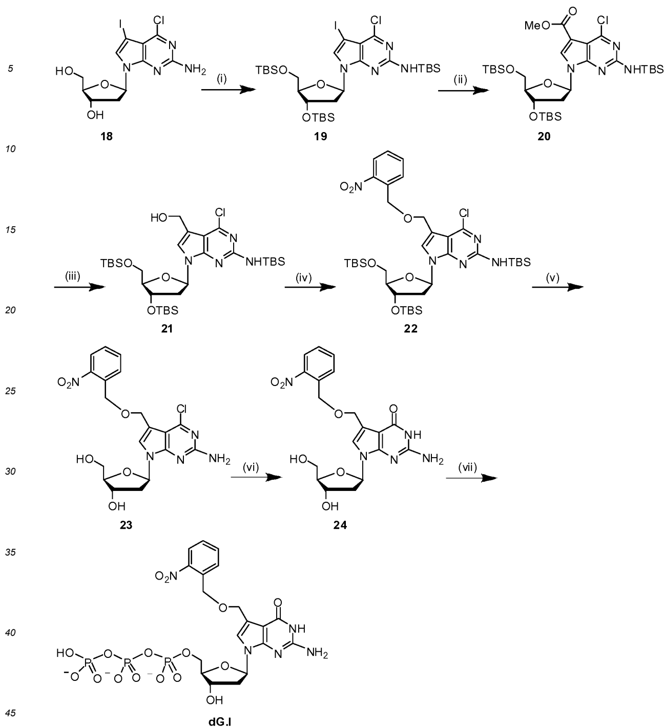
Scheme S12. Synthesis of 7-(2-nitrobenzyloxy)methyl-7-deaza-2'-deoxyguanosine-5'-triphosphate. Reagents and conditions: (i) TBSCl, imidazole, DMF, room temperature, 60%;
