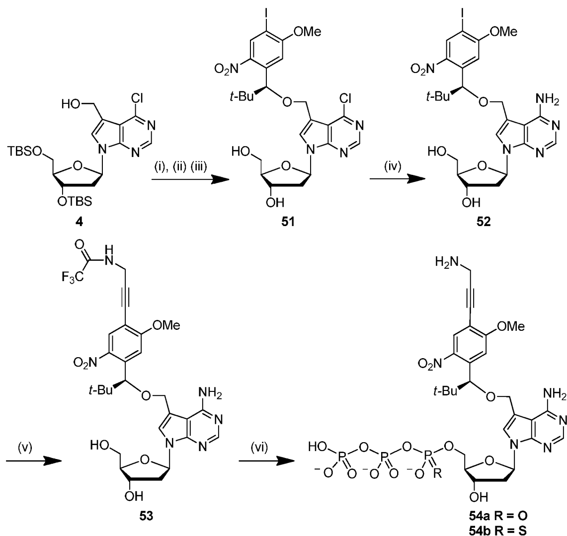
Scheme S25a. Synthesis of dye labeled 7-((S)-1-[4-(3-amino-1-propynyl)-5-methoxy-2-nitrophenyl]-2,2-dimethyl-propyloxy)methyl-7-deaza-2'-deoxyadenosine-5'-triphosphate and 5'- \alpha -thiotriphosphate. Reagents and conditions: (i) MsCl, DMAP, CH 2 Cl 2 , (ii) (S)-1-(4-iodo-5-methoxy-2-nitrophenyl)-2,2-dimethyl-1-propanol, 110°C; (iii) n -Bu 4 NF, THF, room temperature; 29% for three steps; (iv) NH 3 , 1,4-dioxane/MeOH, 100°C, 80%; (v) N -propargyltrifluoroacetamide, Pd(PPh 3 ) 4 (0), CuI, Et 3 N, DMF, 98%; (vi) For 54a : POCl 3 , proton sponge, (MeO) 3 PO, 0°C; ( n -Bu 3 NH) 2 H 2 P 2 O 7 , n -Bu 3 N, DMF; 1 M HNEt 3 HCO 3 ; NH 4 OH. For 54b : PSCl 3 , 2,4,6-collidine, (EtO) 3 PO, 0°C to room temperature; ( n -Bu 3 NH) 2 H 2 P 2 O 7 , n -Bu 3 N, DMF; 1 M HNEt 3 HCO 3 ; NH 4 OH.
