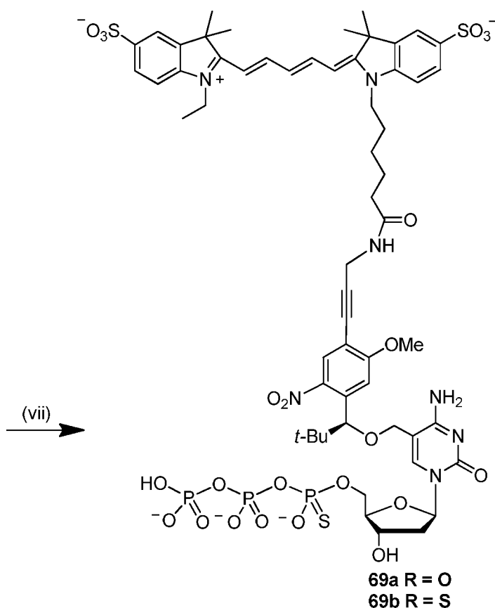
Scheme S28b. (vii) Cy5 NHS, 0.1 M Na 2 CO 3 /NaHCO 3 buffer (pH 9.2).
