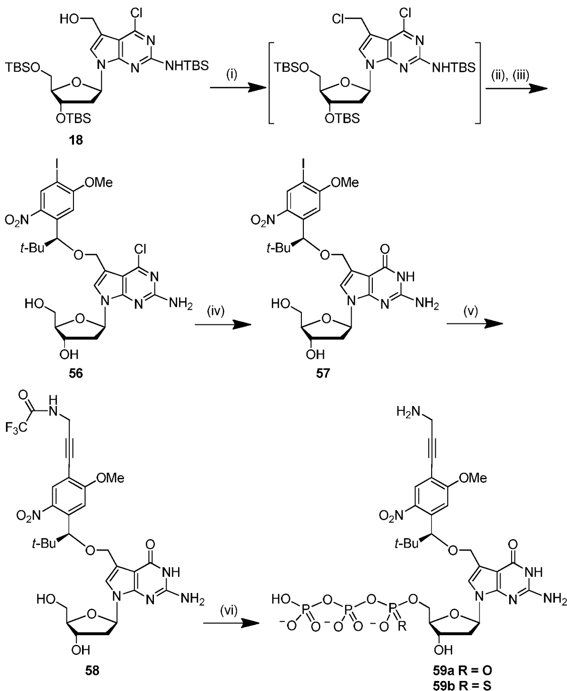
Scheme S26a. Synthesis of dye labeled 7-((S)-1-[4-(3-amino-1-propynyl)-5-methoxy-2-nitrophenyl]-2,2-dimethyl-propyloxy)methyl-7-deaza-2'-deoxyguanosine-5'-triphosphate and 5'- \alpha -thiotriphosphate. Reagents and conditions: (i) MsCl, DMAP, CH 2 Cl 2 , 0°C; (ii) (S)-1-(4-iodo-5-methoxy-2-nitrophenyl)-2,2-dimethyl-1-propanol, 115°C; (iii) n -Bu 4 NF, THF, room
