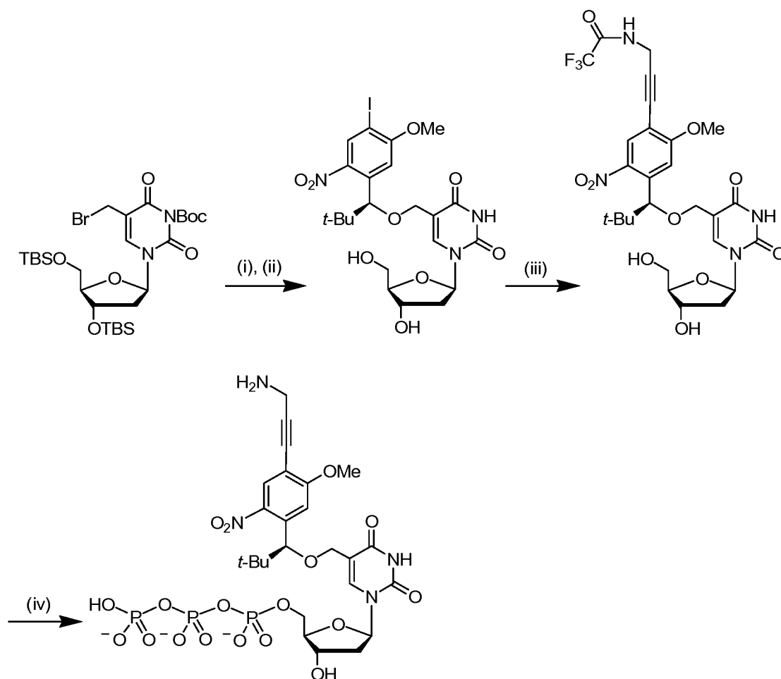
Scheme 3a. Synthesis of dye labeled 5-[(S)-1-(5-methoxy-2-nitrophenyl)-2,2-dimethyl-propyloxy]methyl-2'-deoxyuridine-5'-triphosphate. Reagents and conditions: (i) (S)-1-(4-iodo-5-methoxy-2-nitrophenyl)-2,2-dimethyl-1-propanol, 110^\circ\text{C} ; (ii) \text{NH}_4\text{F} , MeOH, 50^\circ\text{C} ; (iii) N-propargyltrifluoroacetamide, \text{Pd}(\text{PPh}_3)_4(0) , CuI, \text{Et}_3\text{N} , DMF; (iv) \text{POCl}_3 , proton sponge, (\text{MeO})_3\text{PO} , 0^\circ\text{C} ; (n\text{-Bu}_3\text{NH})_2\text{H}_2\text{P}_2\text{O}_7 , n\text{-Bu}_3\text{N} , DMF; 1\text{ M HNEt}_3\text{HCO}_3 ;
