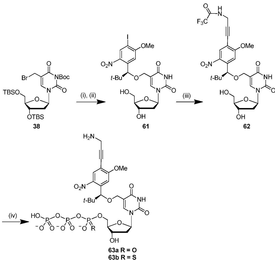
Scheme S27a. Synthesis of dye labeled 5-(( S )-1-[4-(3-amino-1-propynyl)-5-methoxy-2-nitrophenyl]-2,2-dimethyl-propyloxy)methyl-2'-deoxyuridine-5'-triphosphate. Reagents and conditions: (i) ( S )-1-(4-iodo-5-methoxy-2-nitrophenyl)-2,2-dimethyl-1-propanol, 110°C; (ii) NH 4 F, MeOH, 50°C, 28% for two steps; (iii) N -propargyltrifluoroacetamide, Pd(PPh 3 ) 4 (0), CuI, Et 3 N, DMF, 90%; (iv) For 63a : POCl 3 , proton sponge, (MeO) 3 PO, 0°C; ( n -Bu 3 NH) 2 H 2 P 2 O 7 , n -Bu 3 N, DMF; 1 M HNEt 3 HCO 3 ; NH 4 OH. For 63b : PSCl 3 , 2,6-lutidine, (EtO) 3 PO, 0°C to room temperature; ( n -Bu 3 NH) 2 H 2 P 2 O 7 , n -Bu 3 N, DMF; 1 M HNEt 3 HCO 3 ; NH 4 OH.
