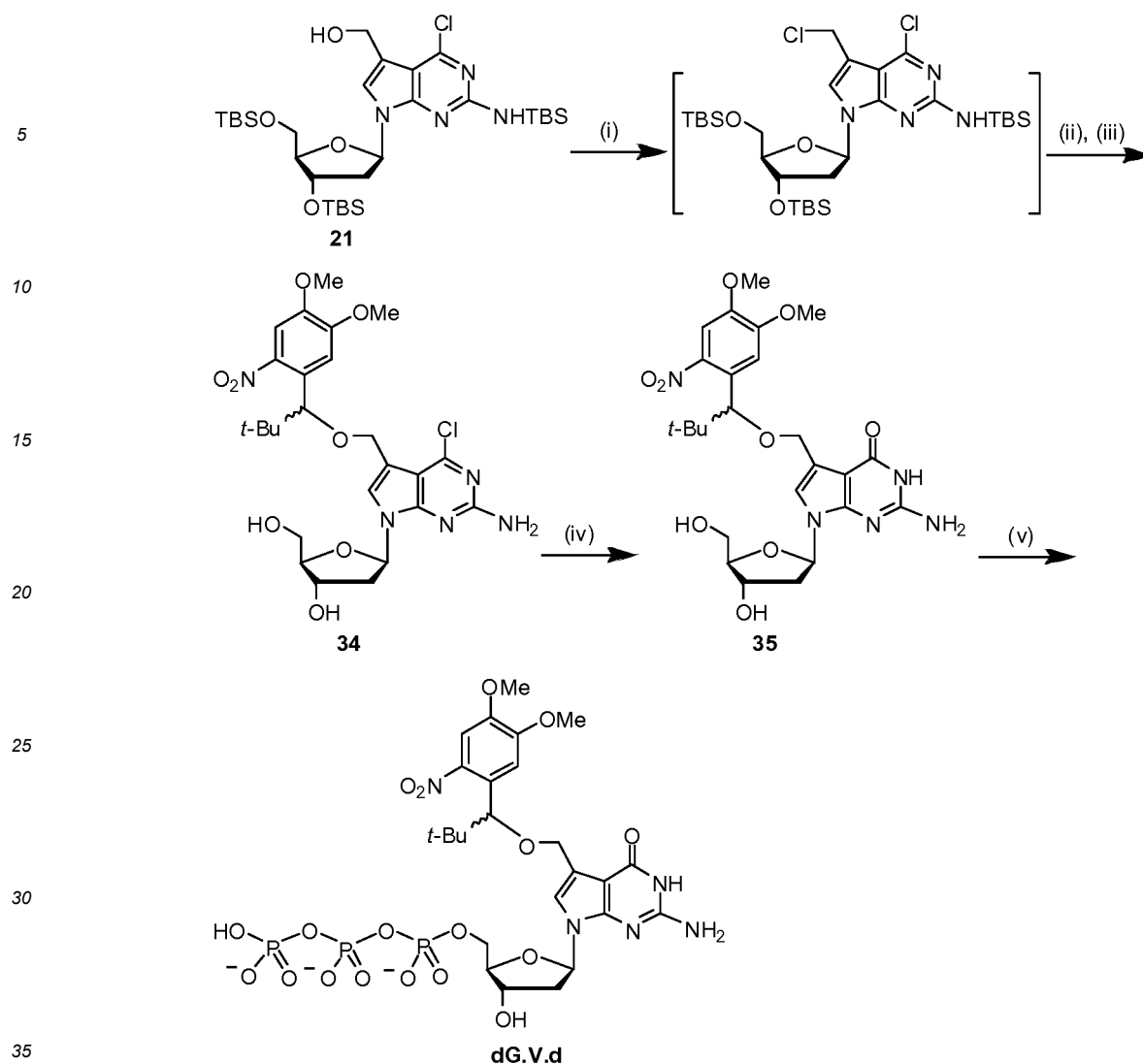
Scheme S17. Synthesis of 7-[1-(4,5-dimethoxy-2-nitrophenyl)-2,2-dimethyl-propyloxy]methyl-7-deaza-2'-deoxyguanosine-5'-triphosphate. Reagents and conditions: (i) MsCl, DMAP, CH 2 Cl 2 , 0°C; (ii) racemic ( R/S )-1-(4,5-dimethoxy-2-nitrophenyl)-2,2-dimethyl-1-propanol, 115°C; (iii) n -Bu 4 NF, THF, room temperature, 23% for three steps; (iv) syn-pyridine-2-aldoxime, 1,1,3,3-tetramethyl guanidine, dioxane/DMF, 70°C, 68%; (v) POCl 3 , proton sponge, (MeO) 3 PO, 0°C; ( n -Bu 3 NH) 2 H 2 P 2 O 7 , n -Bu 3 N, DMF; 1 M HNEt 3 HCO 3 .
