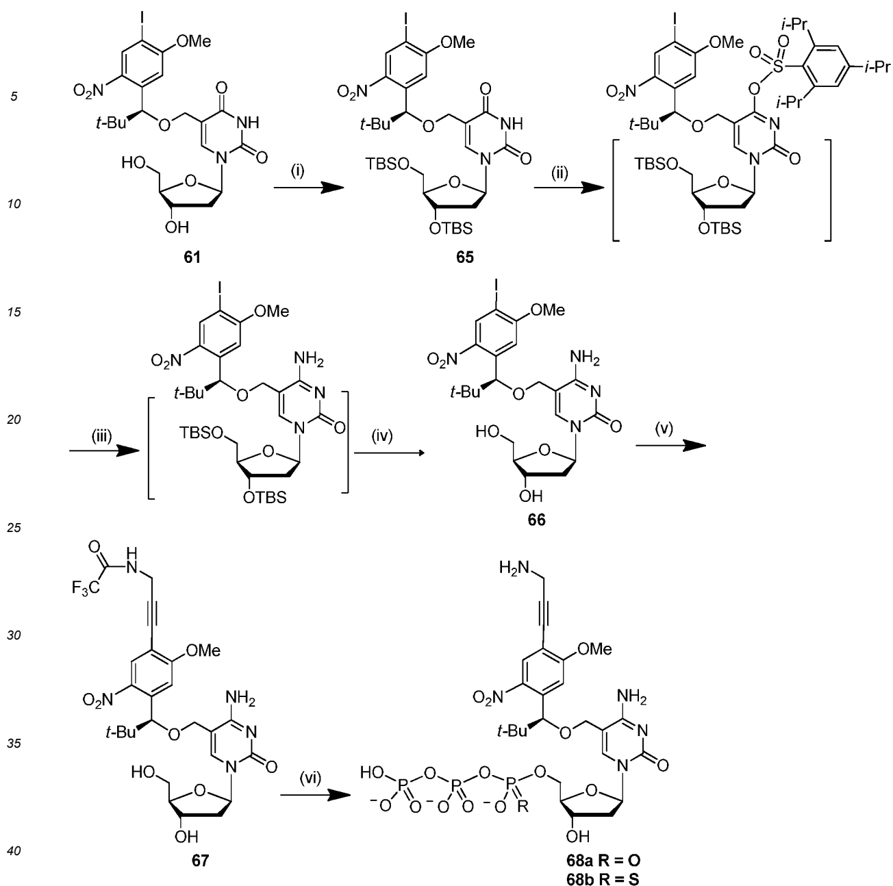
Scheme S28a. Synthesis of dye labeled 5-(( S )-1-[4-(3-amino-1-propynyl)-5-methoxy-2-nitrophenyl]-2,2-dimethyl-propyloxy)methyl-2'-deoxycytidine-5'-triphosphate.
