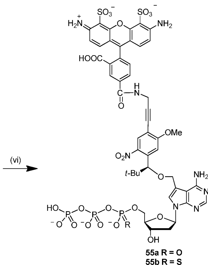
Scheme S25b. (vi) Alexa Fluor 488 NHS, 0.1 M Na 2 CO 3 /NaHCO 3 buffer (pH 9.2).
