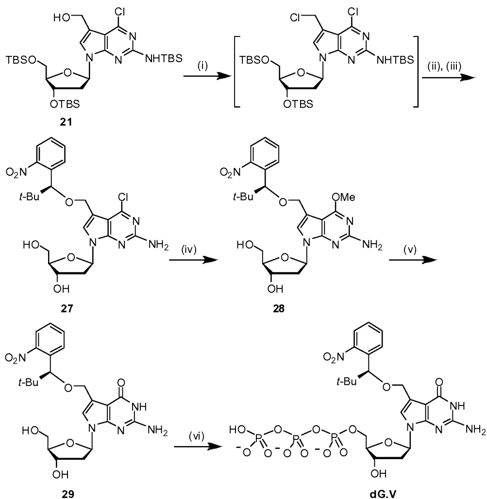
Scheme S14. Synthesis of 7-[( S )-1-(2-nitrophenyl)-2,2-dimethyl-propyloxy]methyl-7-deaza-2'-deoxy-guanosine-5'-triphosphate. Reagents and conditions: (i) MsCl, DMAP, CH 2 Cl 2 , 0°C; (ii) ( S )-1-(2-nitrophenyl)-2,2-dimethyl-1-propanol, 115°C; (iii) n -Bu 4 NF, THF, room temperature, 35% for three steps; (iv) NaOMe, MeOH, reflux, 74%; (v) 1,4-dioxane, 2 M NaOH, reflux, 33%; (vi) POCl 3 , proton sponge, (MeO) 3 PO, 0°C; ( n -Bu 3 NH) 2 H 2 P 2 O 7 , n -Bu 3 N, DMF; 1 M HNet 3 HCO 3 .
