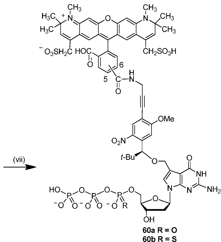
Scheme S26b. (vii) Alexa Fluor 594 NHS, 0.1 M Na 2 CO 3 /NaHCO 3 buffer (pH 9.2).
