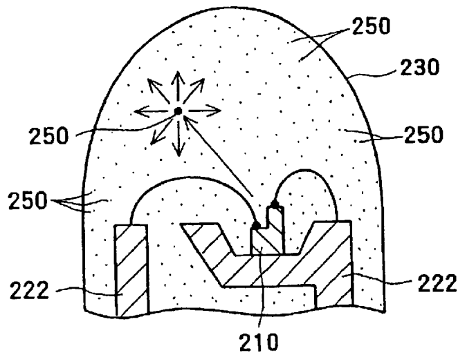
FIG. 50 PRIOR ART
