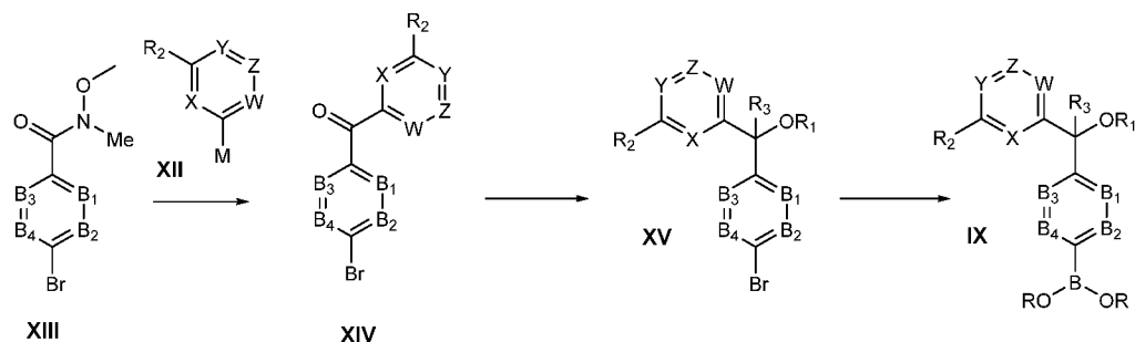
Route 2
