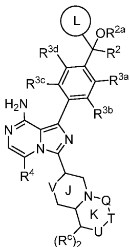
Formula I
