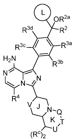
Formula I
