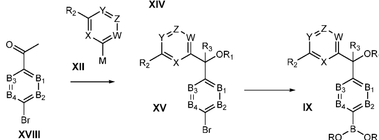
Route 3
