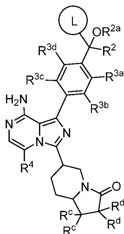
Formula Ia
