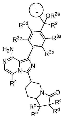
Formula Ia
