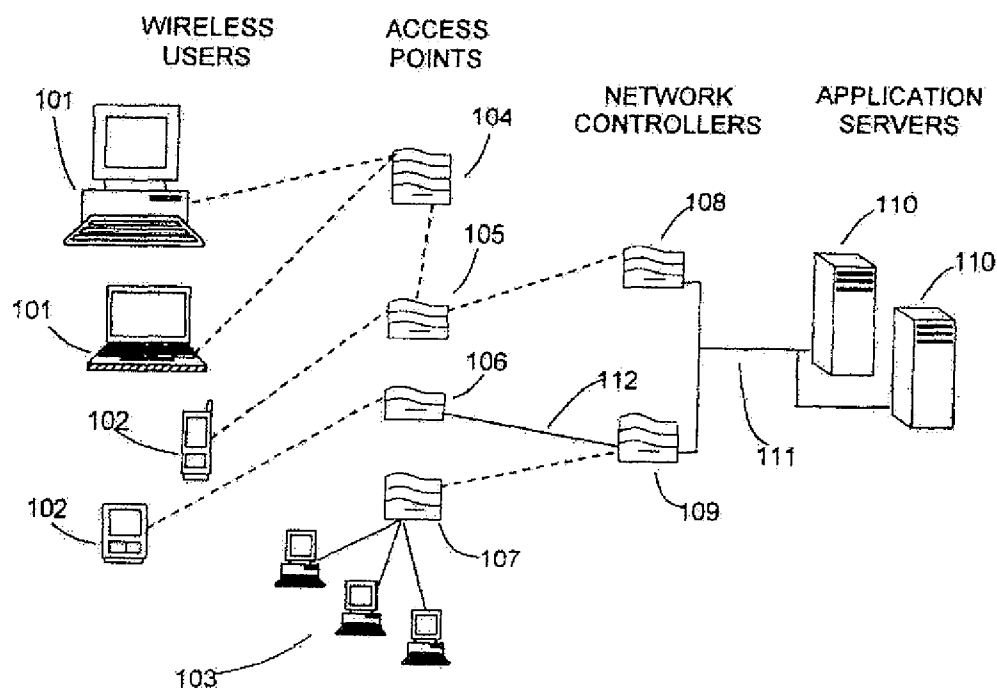
FIG. 1A WIRELESS LOCAL AREA NETWORK SYSTEM
