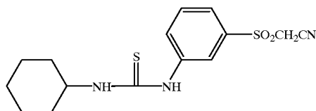
Synthetic Intermediate 1
