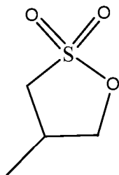
Compound 6,
