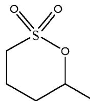
Compound 7,
