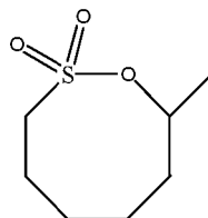
Compound 9, and
