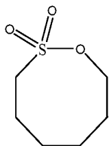
Compound 4,
