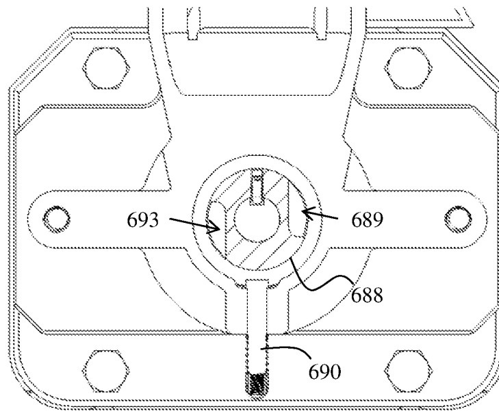
Auger Lock Bolt- Free Position
