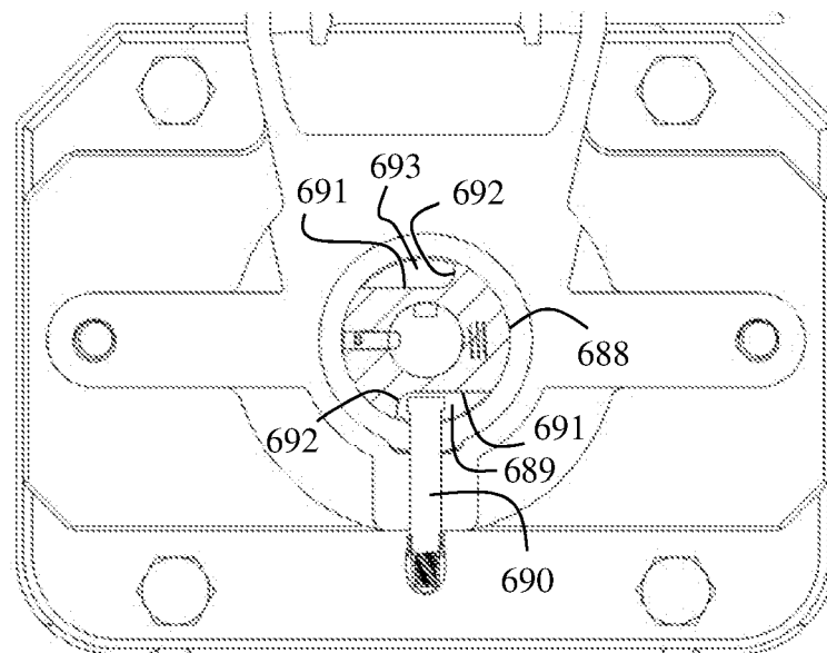
Auger Lock Bolt- Locked Position
