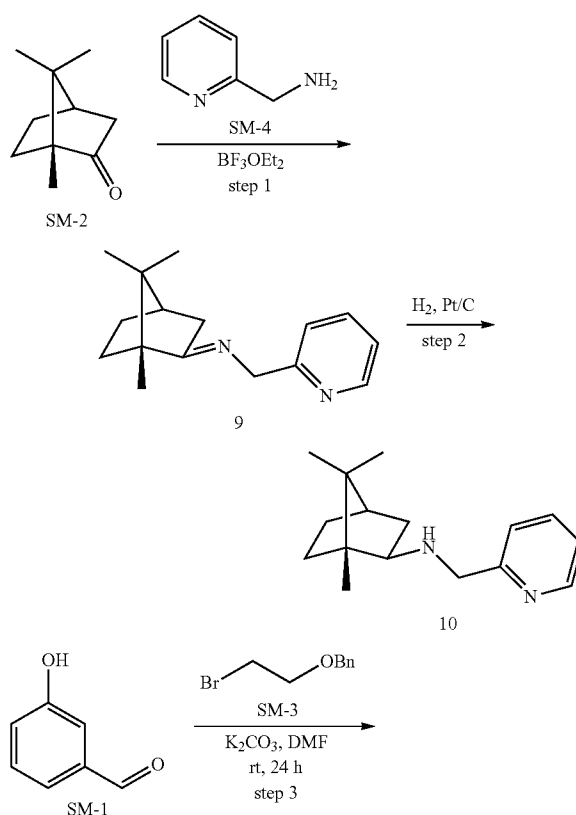
Scheme 5
