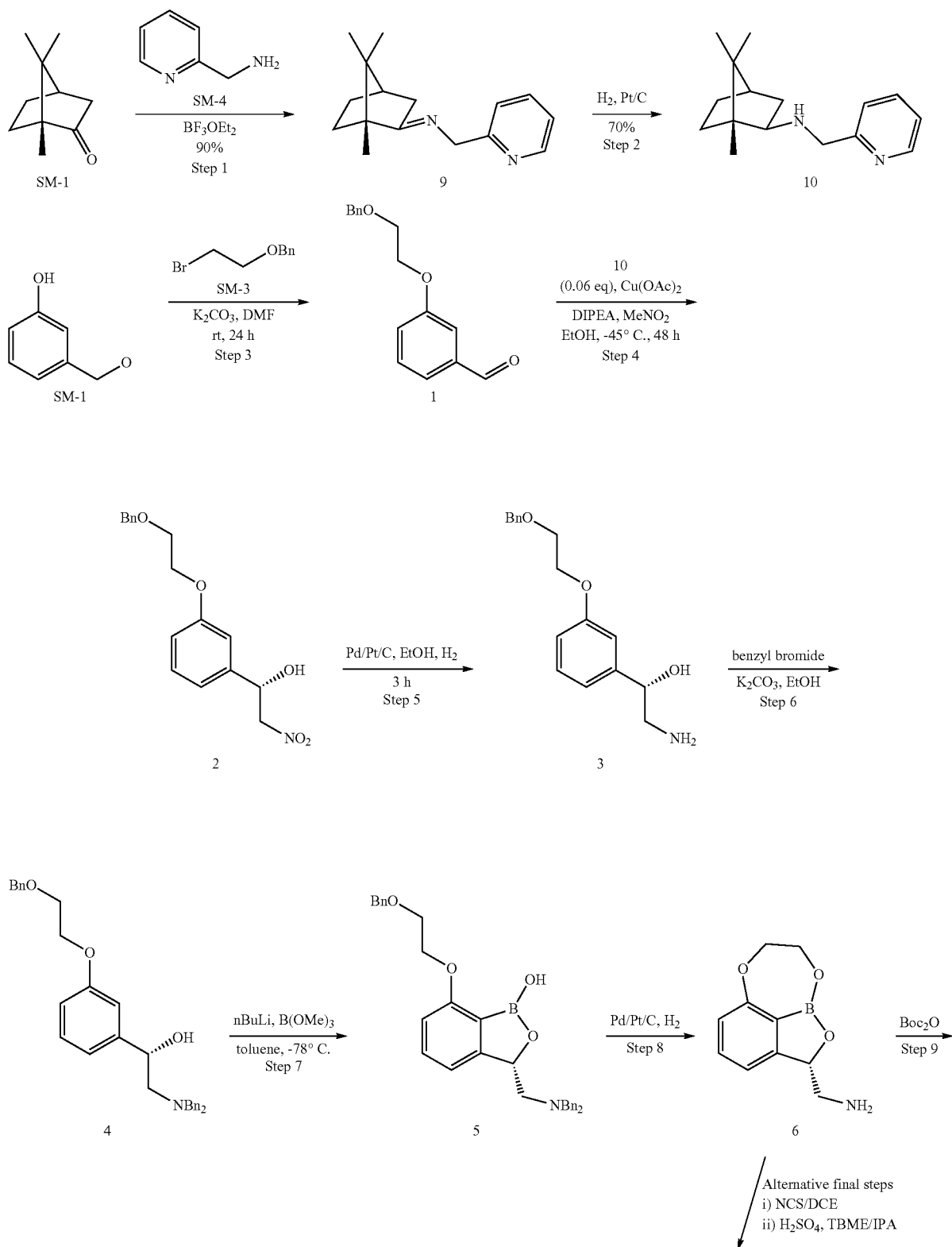
Scheme 6
