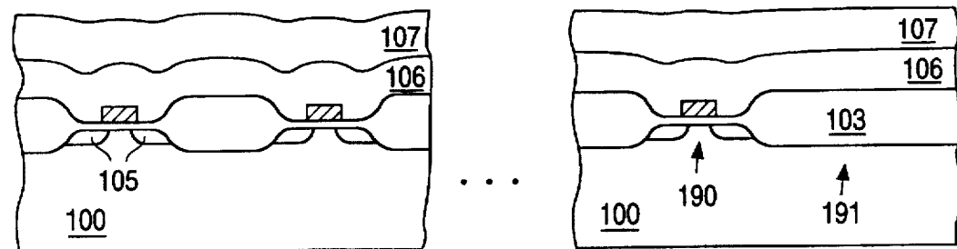
FIG. 1d (PRIOR ART)
