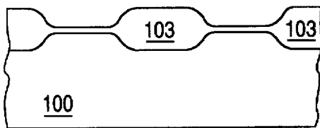
FIG. 2b (PRIOR ART)
