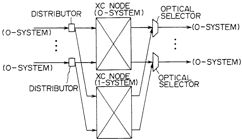
TYPE A (NODE IS DUPLEXED)
