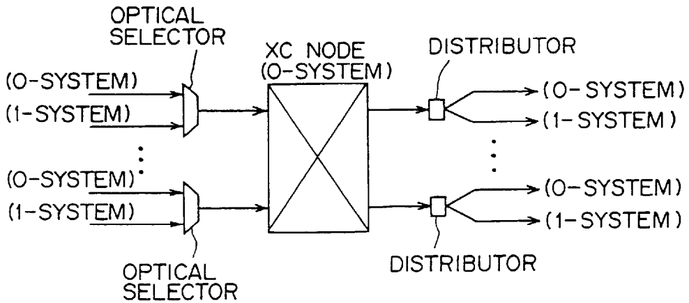
TYPE B (TRANSMISSION LINE IS DUPLEXED)
