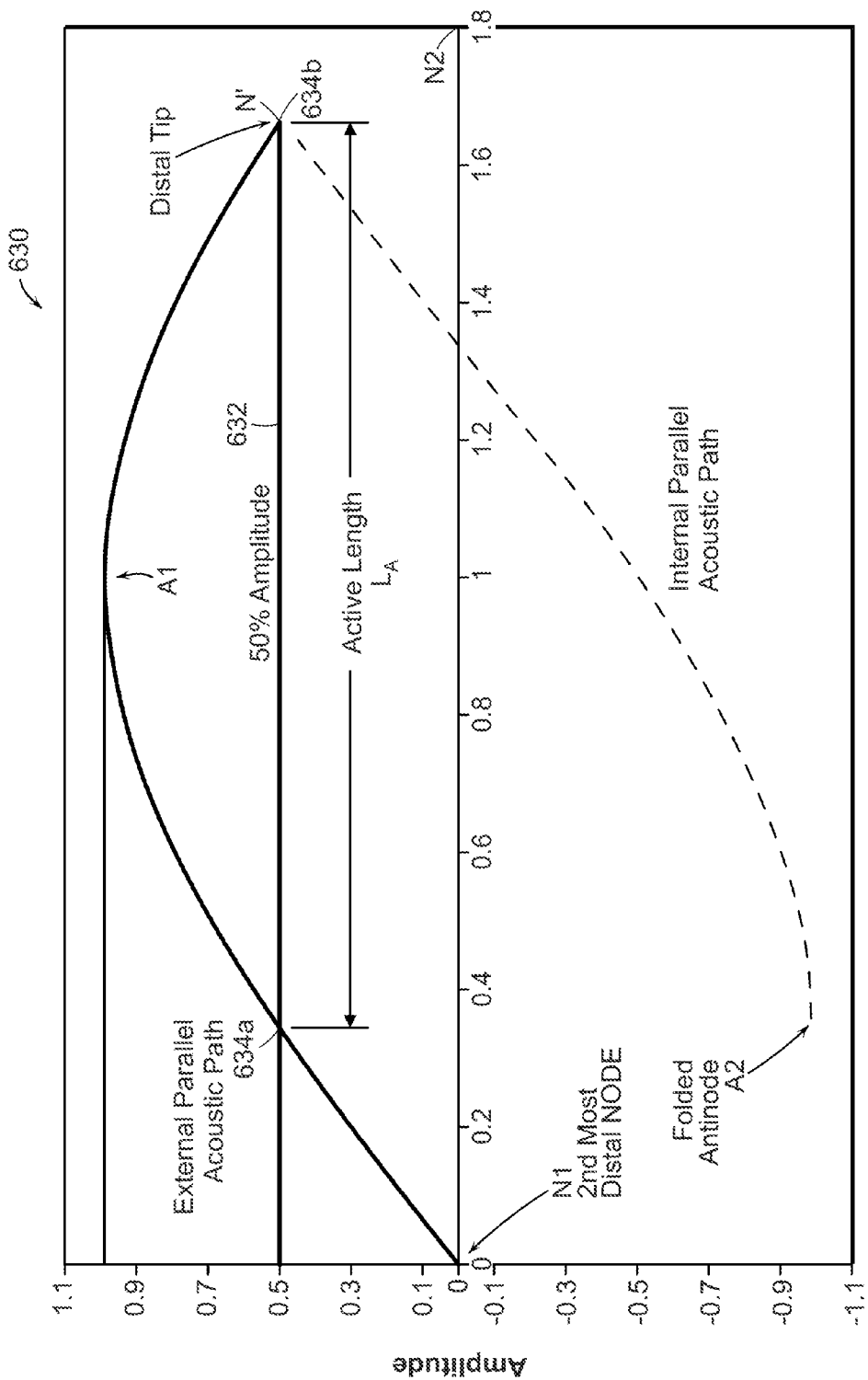
Quarter Wavelengths
