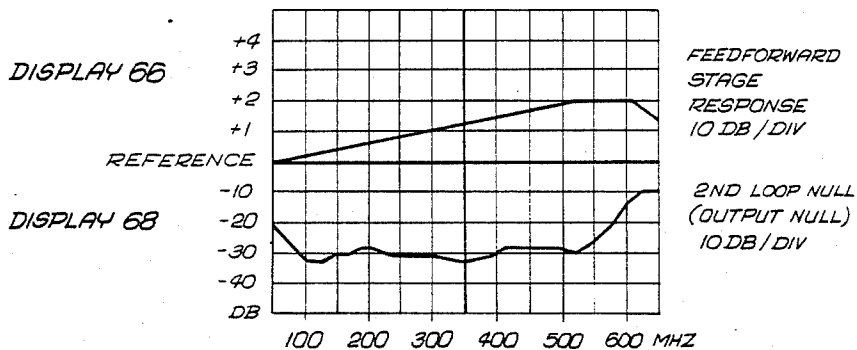
RESPONSE AND OUTPUT NULL PATTERN
