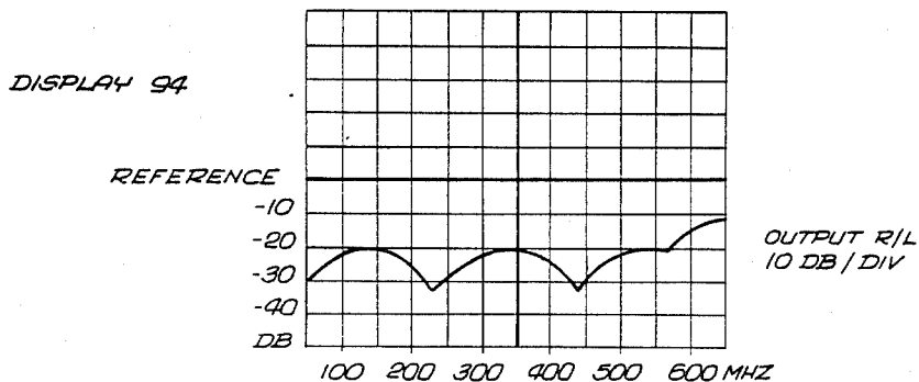
OUTPUT RETURN LOSS
