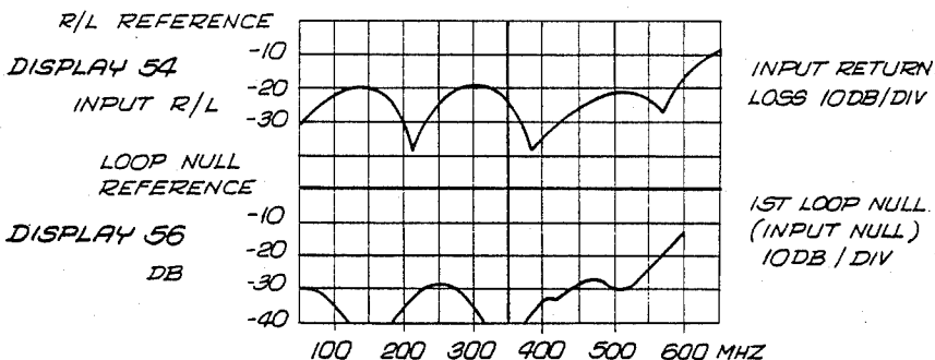
INPUT RETURN LOSS AND INPUT NULL PATTERN
