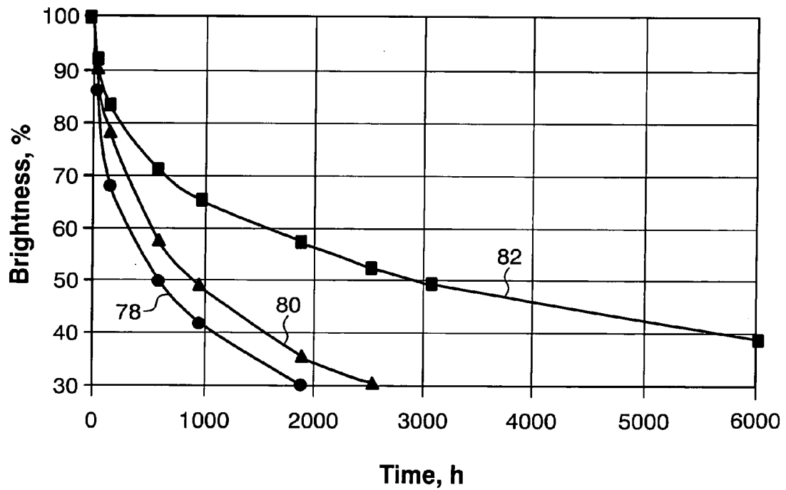
Life Time of EL Light Source
