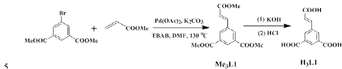
Scheme S1. The synthesis procedure for \text{H}_3\text{L1} .
