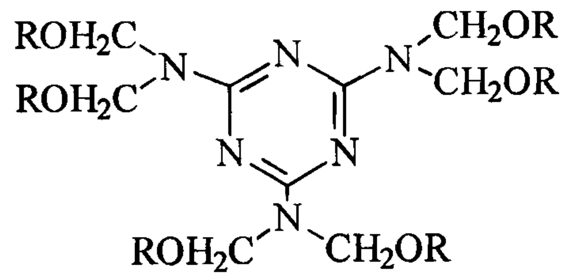
melamine formaldehyde
