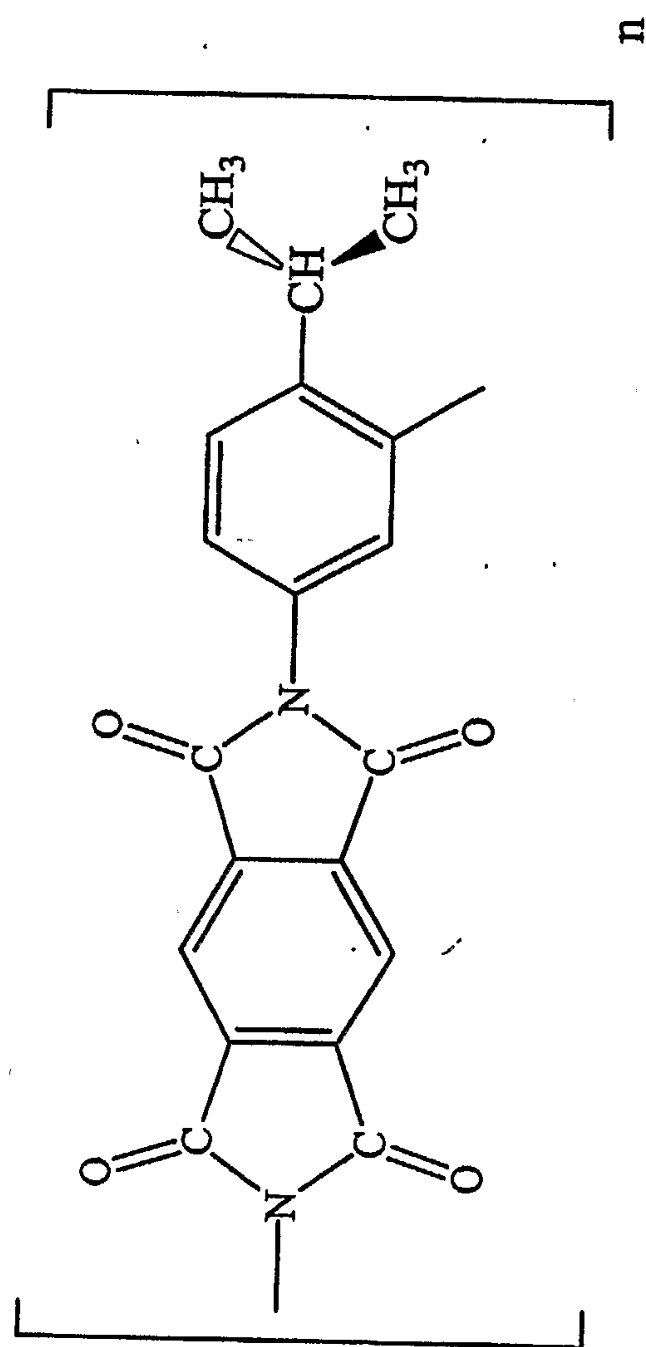
poly(PMDA+4-isopropyl-m-phenylenediamine)imide
