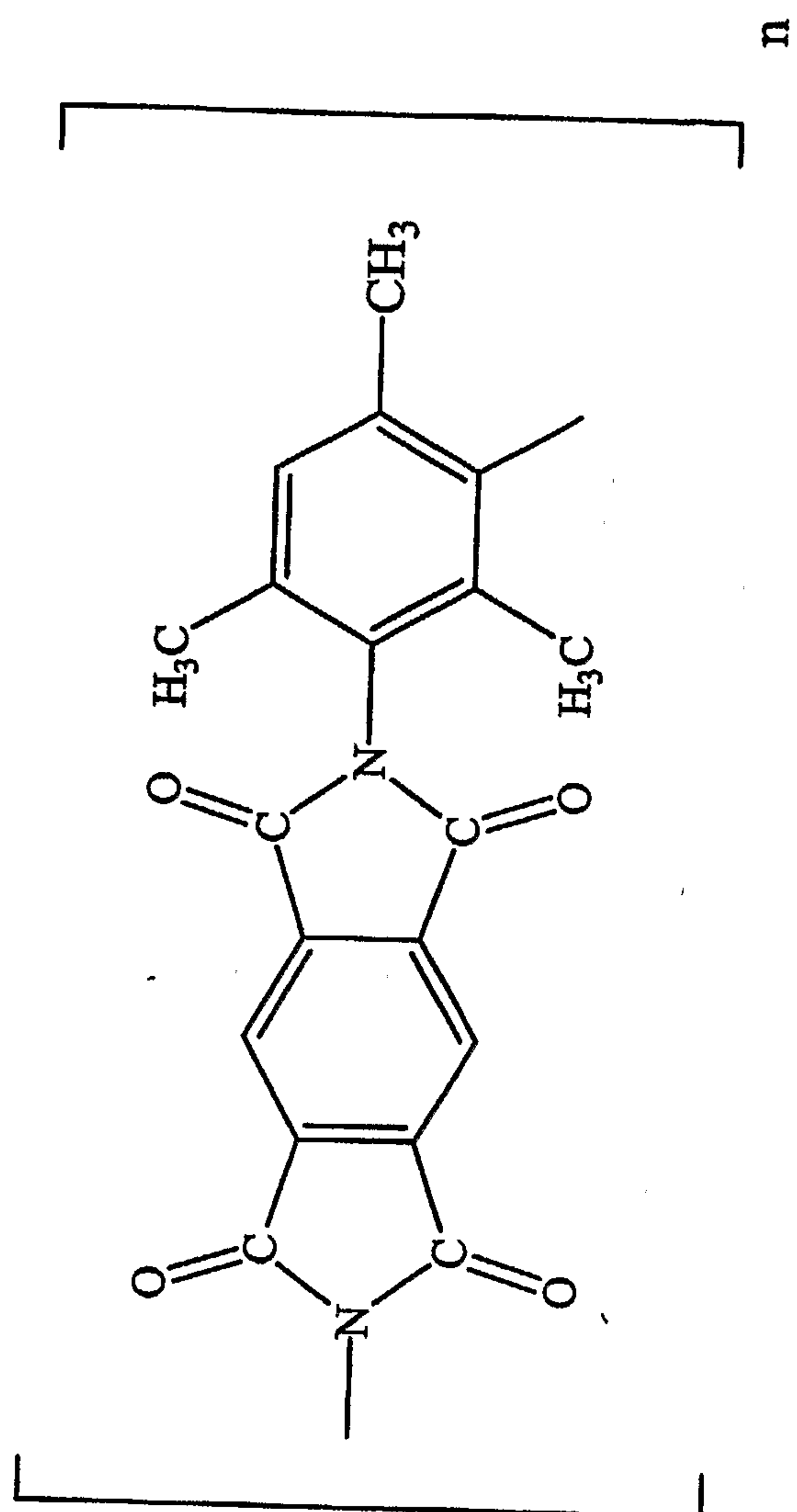
poly(PMDA+DAMs)imide
