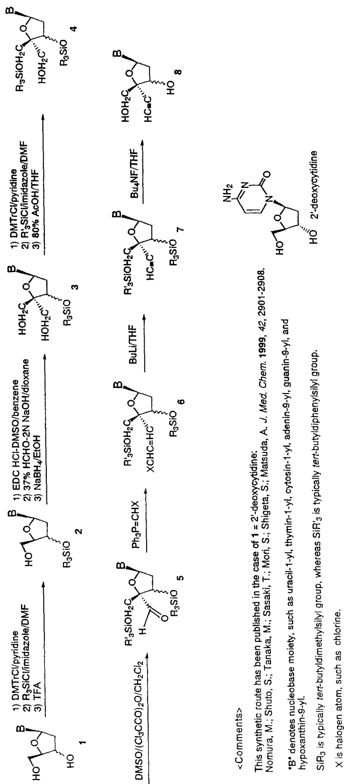
Scheme 1. Synthesis of 4'-ethynyl-2'-deoxynucleosides from 2'-deoxynucleosides
