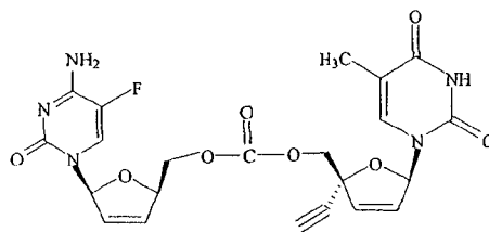
BLFd4C and TKD-4-114 Dinucleoside Carbonate
