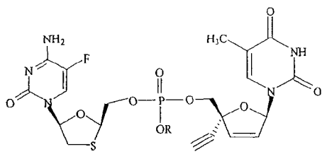
FTC and TKD-4-114 Dinucleoside Phosphate
