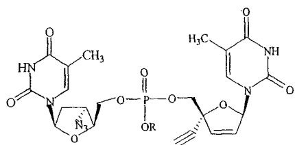
AZT and TKD-4-114 Dinucleoside Phosphate
