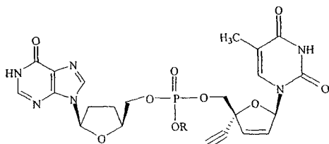
ddI and TKD-4-114 Dinucleoside Phosphate
