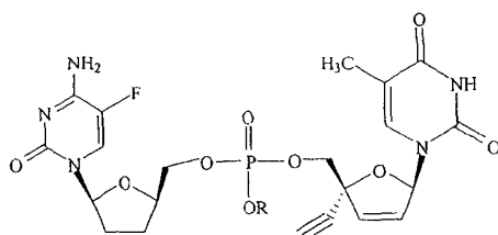
BLFddC and TKD-4-114 Dinucleoside Phosphate
