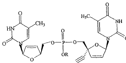
d4T and TKD-4-114 Dinucleoside Phosphate
