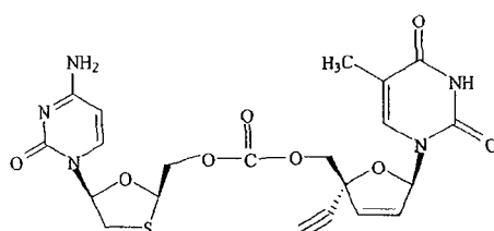
3TC and TKD-4-114 Dinucleoside Carbonate
