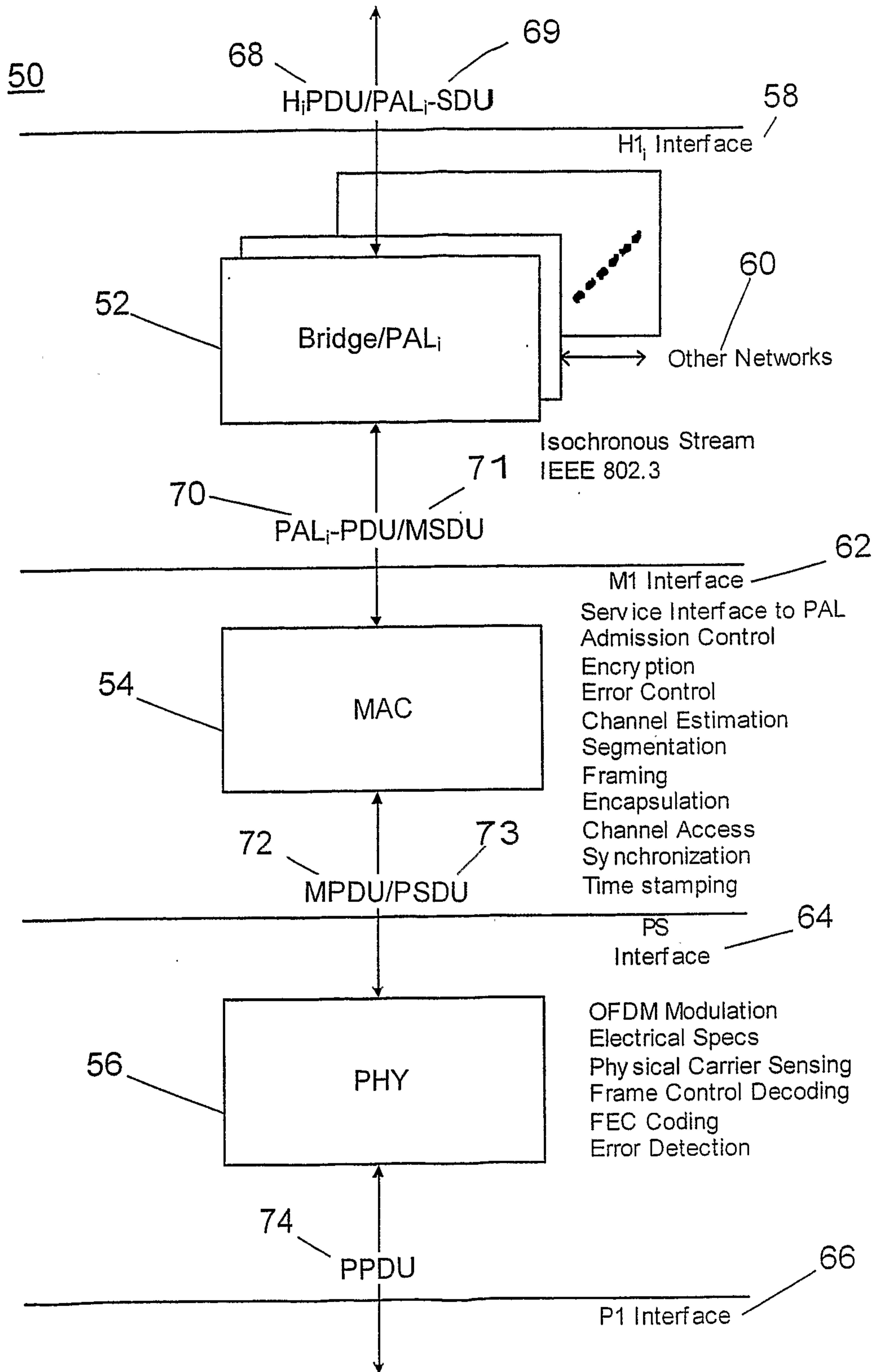
FIG. 2 Reference Network Architecture
