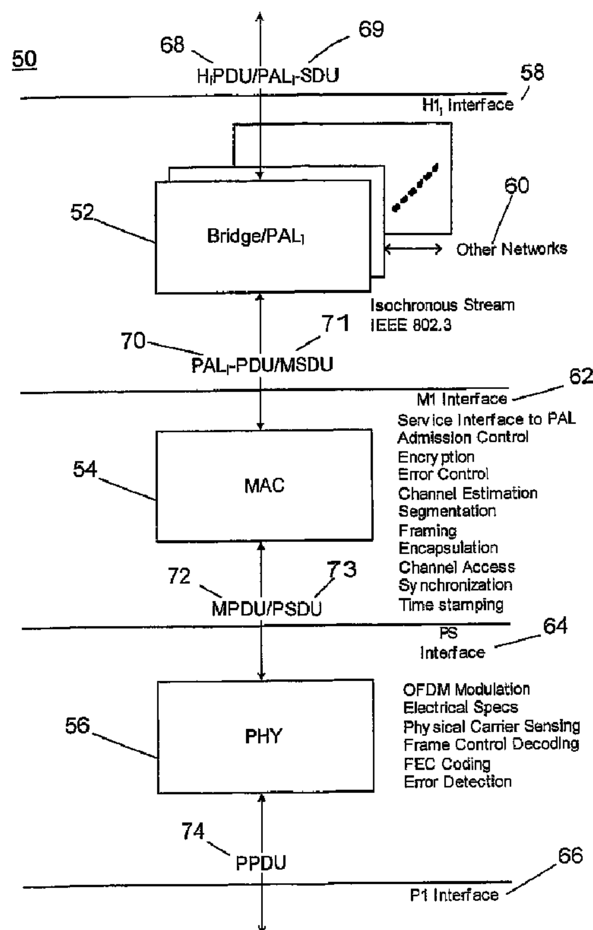
Reference Network Architecture
