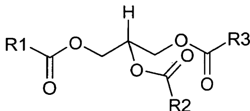
Formel III
