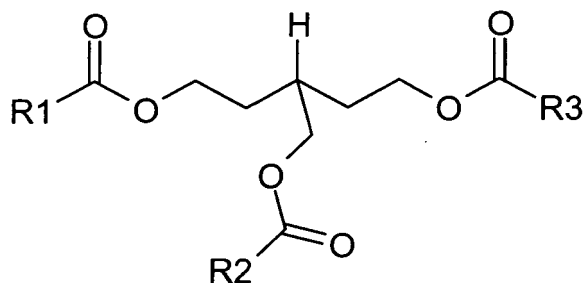
Formel II
