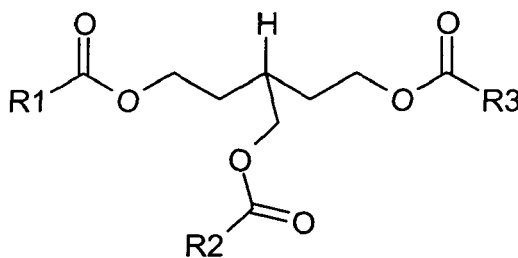
Formel II
