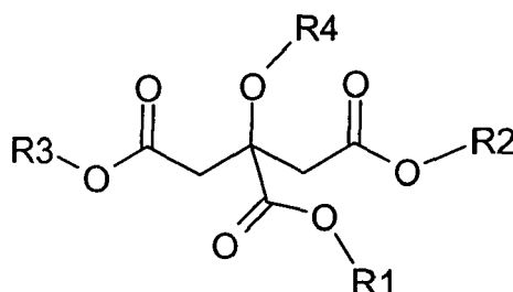
Formel I
