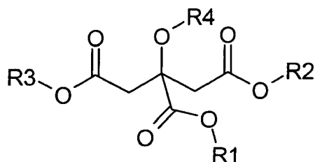
Formel I
