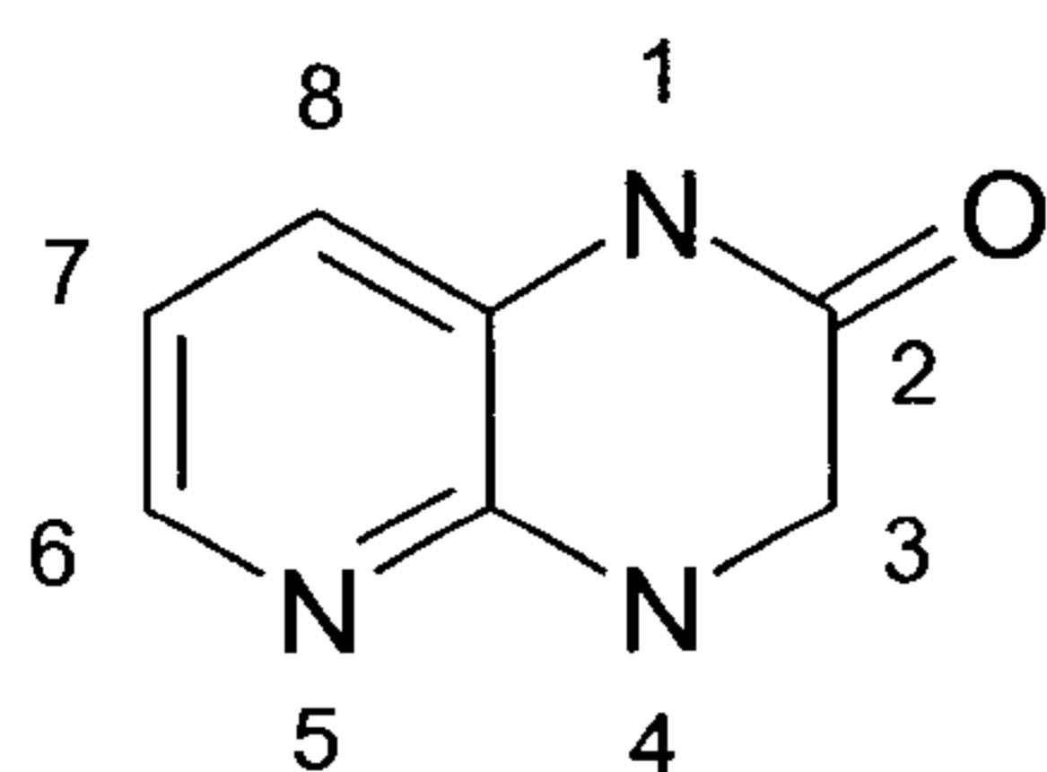
3,4-dihydropyrido[2,3-b]pyrazin-2(1H)-one one
