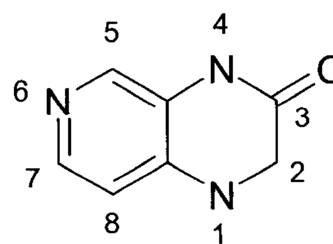
1,4-dihydropyrido[3,4-b]pyrazin-3(2H)-
