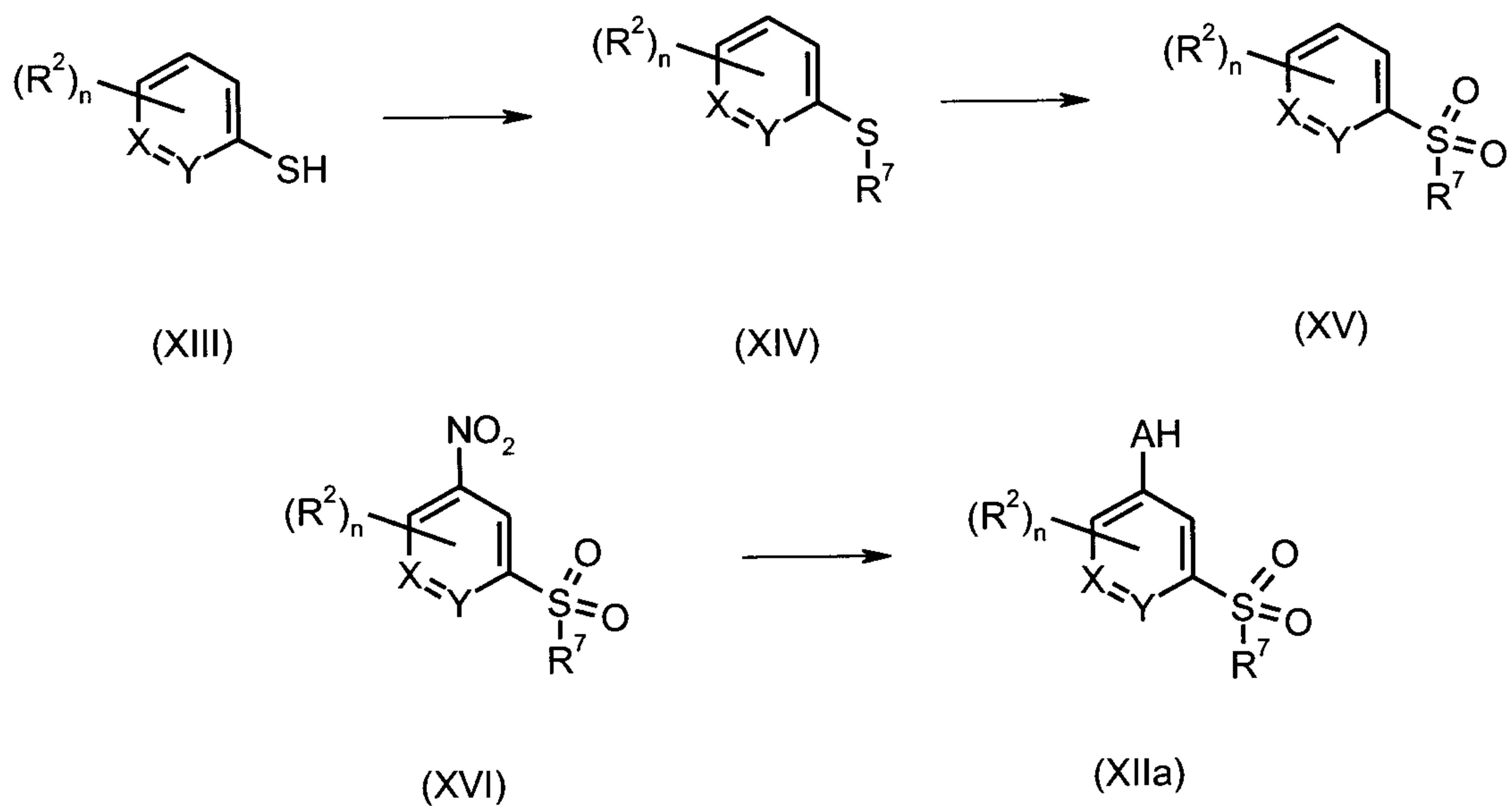
Scheme 4: Preparation of intermediates of the formula (XIIa) from compounds of the formulae (XVI).
