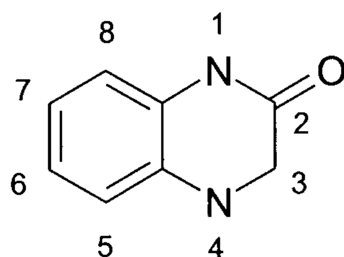
3,4-dihydroquinoxalin-2(1H)-one
