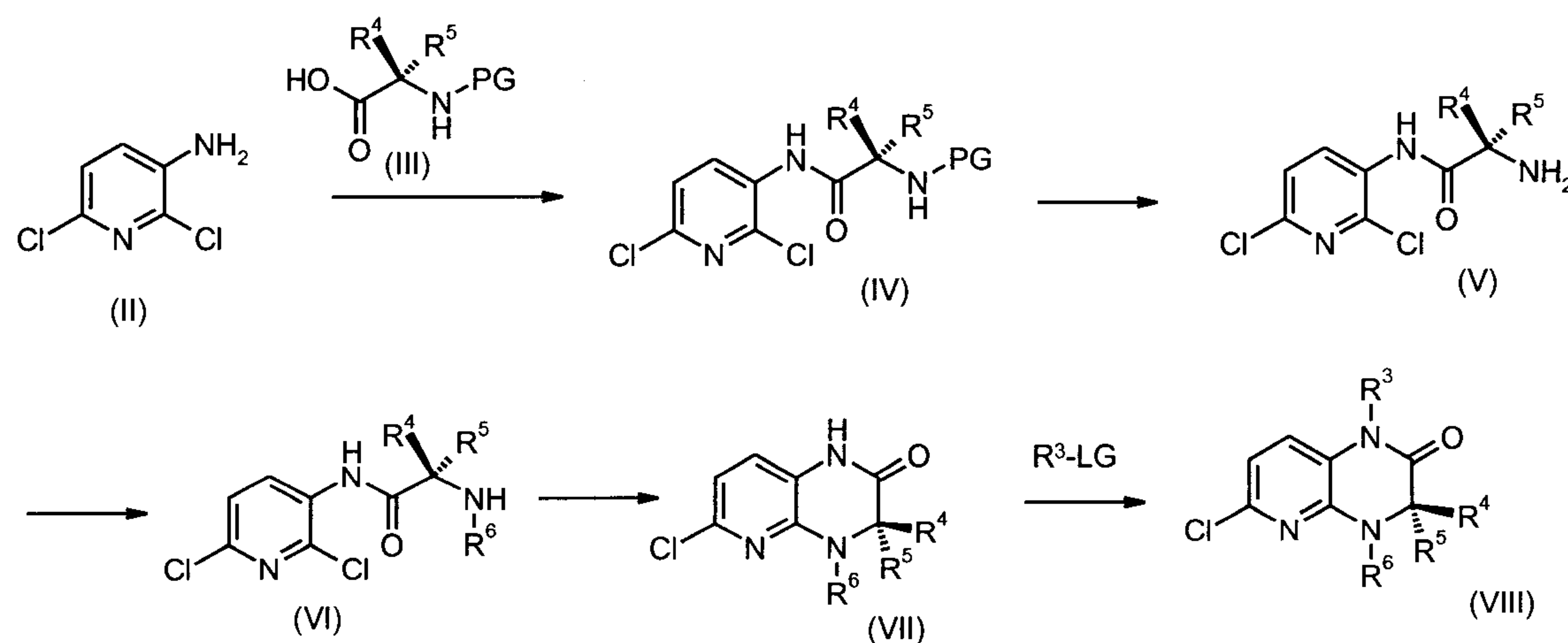
Scheme 1: Synthesis of intermediates of the formula (VIII) from 3-amino-2,6-dichloropyridine (II).
