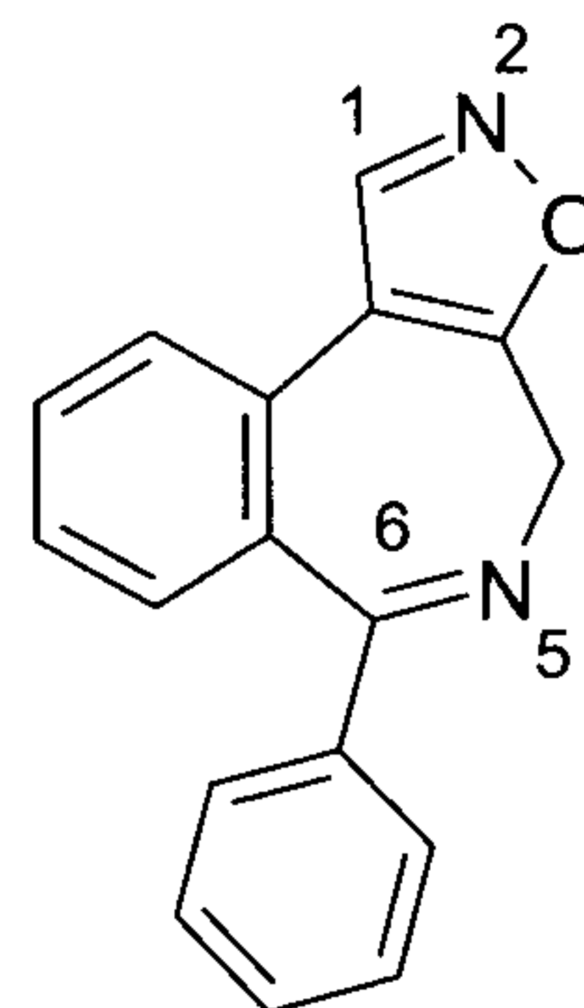
6-phenyl-4H-[1,2]isoxazolo [5,4-d][2]benzazepine
