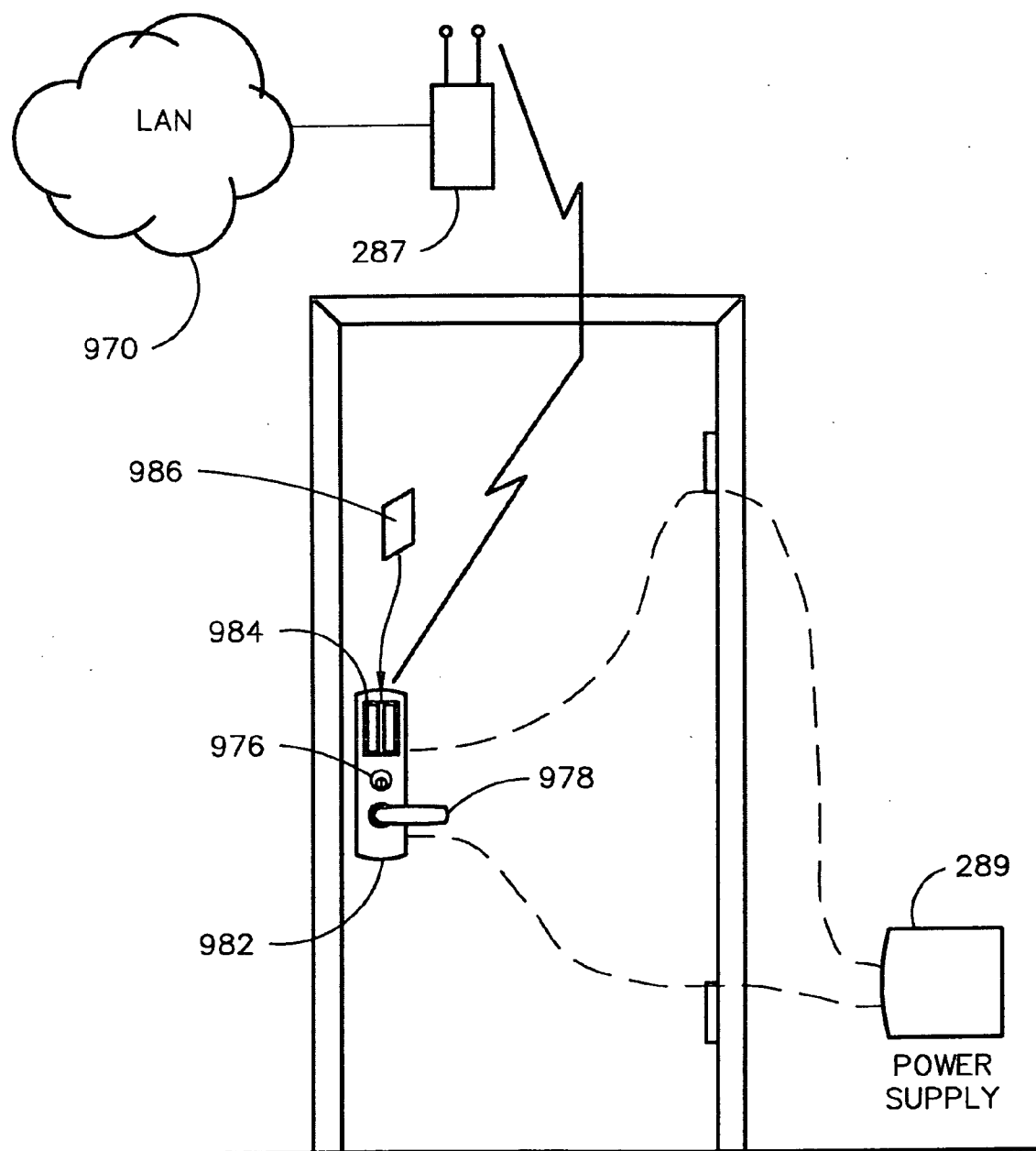
WIRELESS SWIPE CARD MORTISE LOCK
