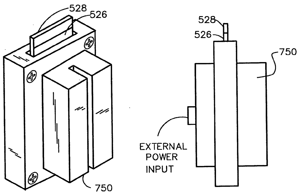
MAG STRIP READER
