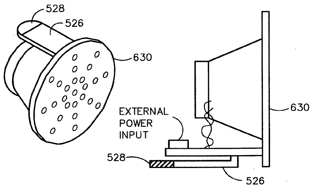
LOUDSPEAKER WITH AMPLIFIER
