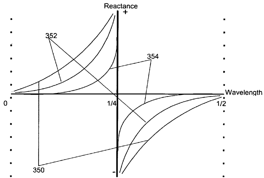
FIG. 16 PRIOR ART
