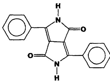
(formula II)
