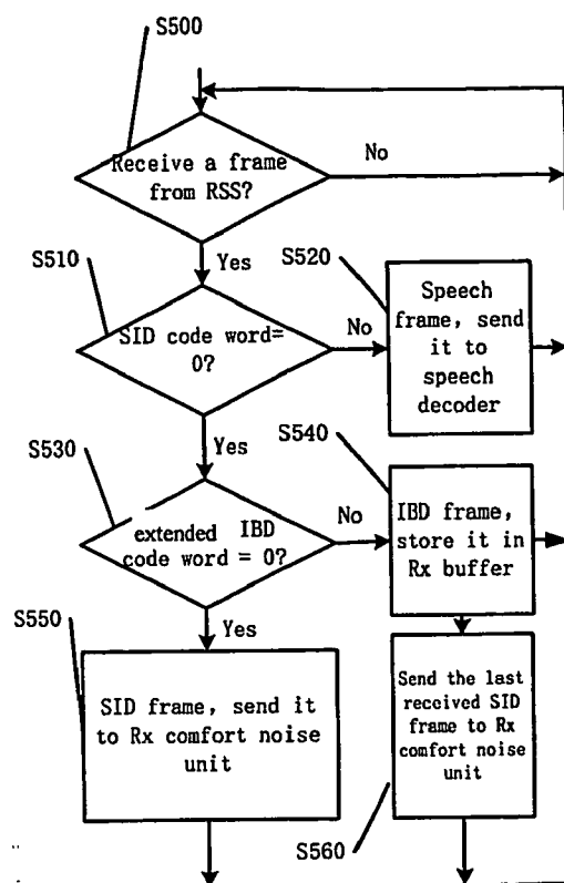
Mobile terminal as receiver
