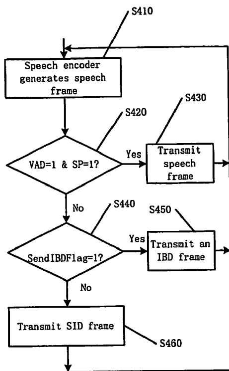
Mobile terminal as sender
