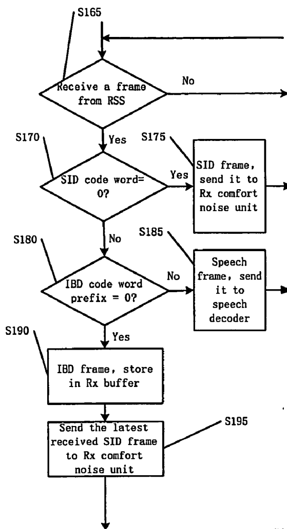
Mobile terminal as receiver
