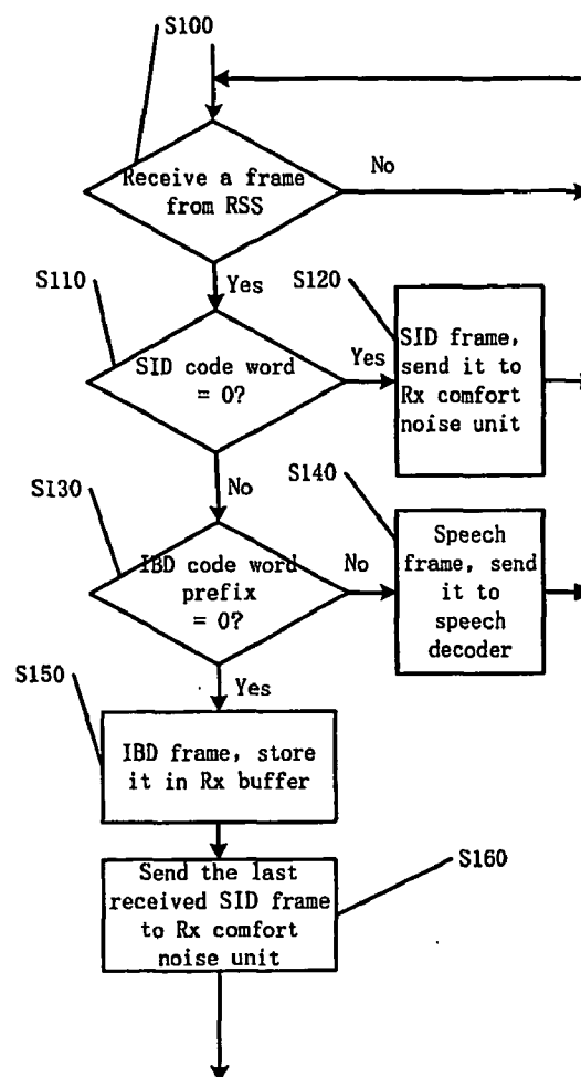
Mobile terminal as receiver
