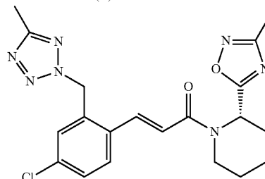
(S)-stereoisomer
