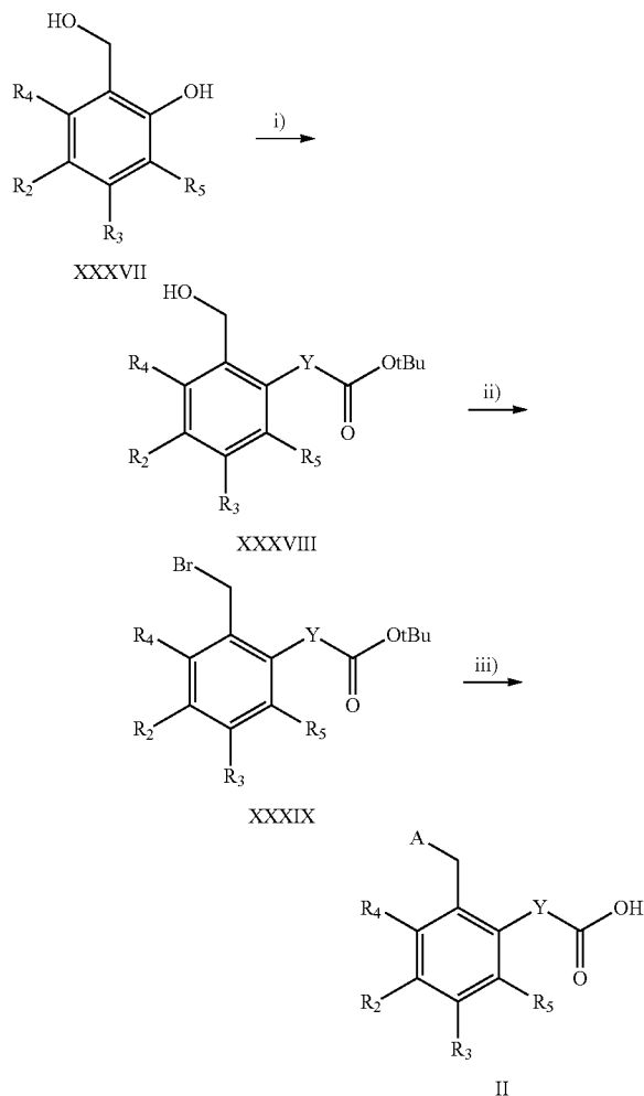
Scheme 20
