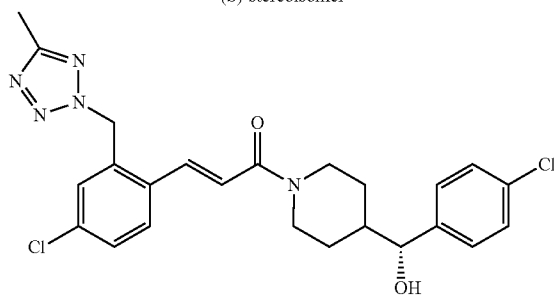
(R)-stereoisomer
