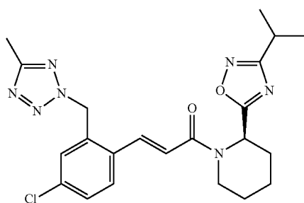
(R)-stereoisomer
