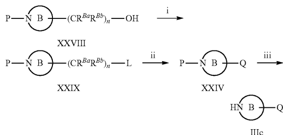
Scheme 16
