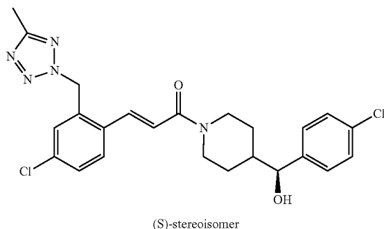
(S)-stereoisomer
