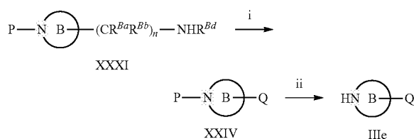
Scheme 18
