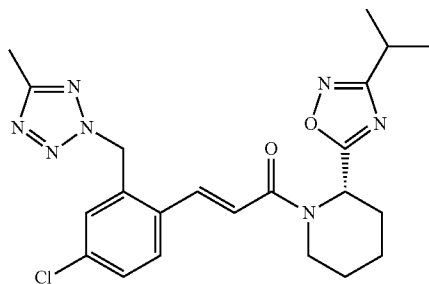
(S)-stereoisomer
