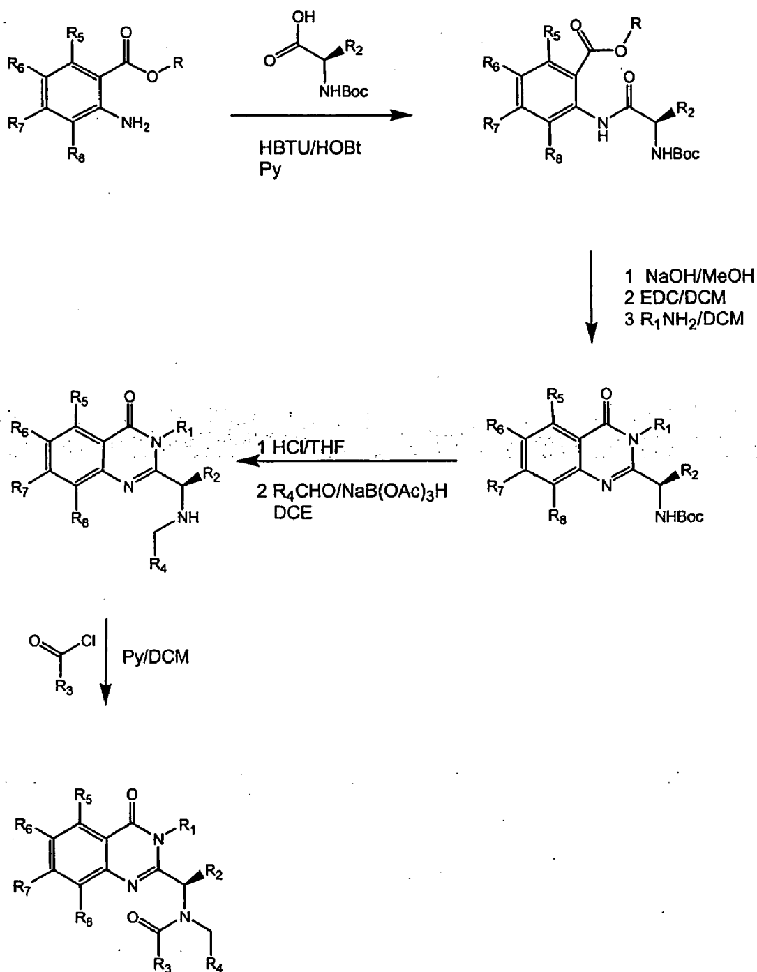
Figure 4: Asymmetric Synthesis
