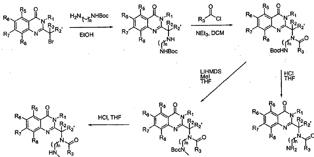
Figure 5d: Primary and Secondary Amine R_4 Synthesis
