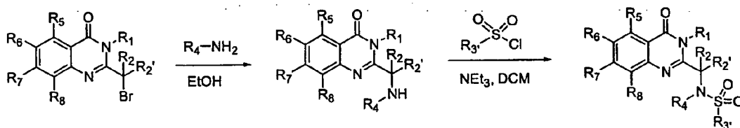
Figure 5b: Carbamate Synthesis
