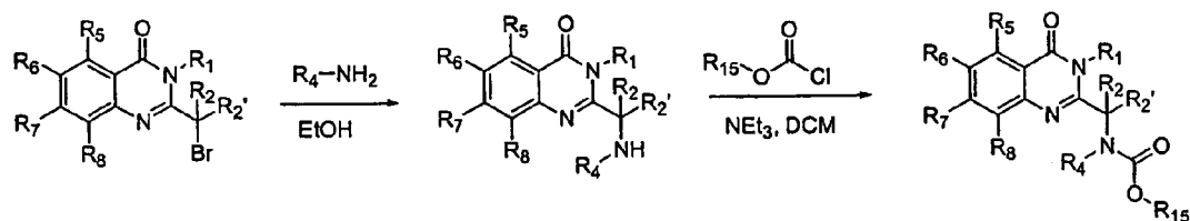
Figure 5c: Urea Synthesis
