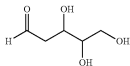
2-Deoxy-D-ribose
