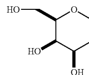
D-Galactal
