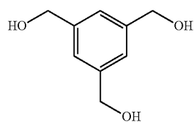
1,3,5-Tri(hydroxymethyl)benzene
