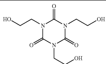
1,3,5-Tris(2-hydroxyethyl)-Cyanuric acid
