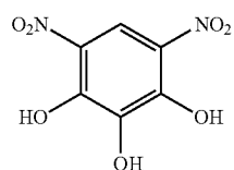
4,6-Nitropyrogallol
