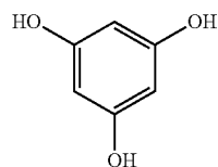
1,3,5-Trihydroxyl-benzene
