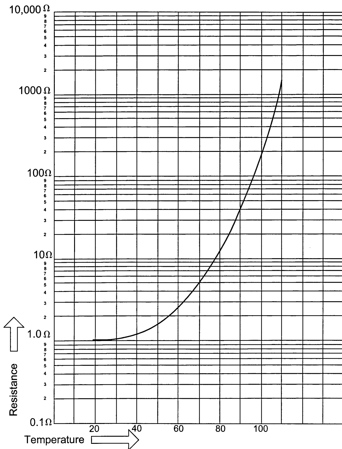
PTC Heaters Resistance vs. Temperature
